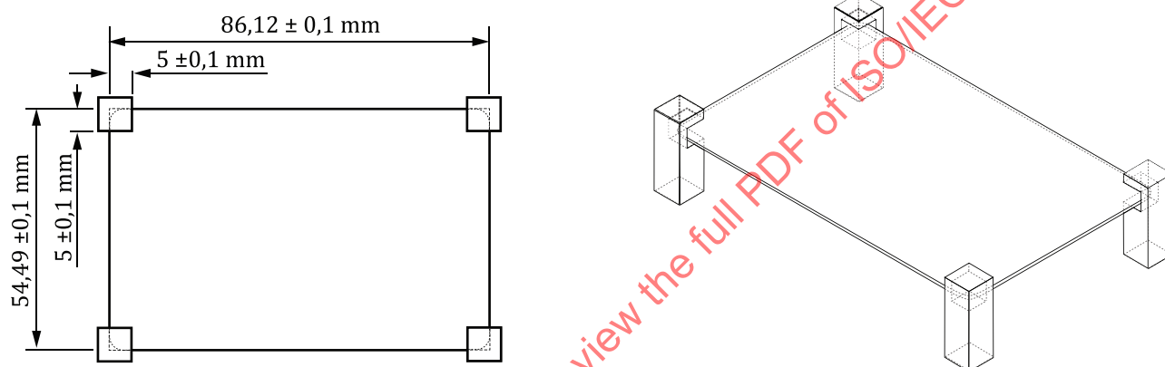
Figure D.5 — ICC holding geometry with ICC (top view and 3D view)
