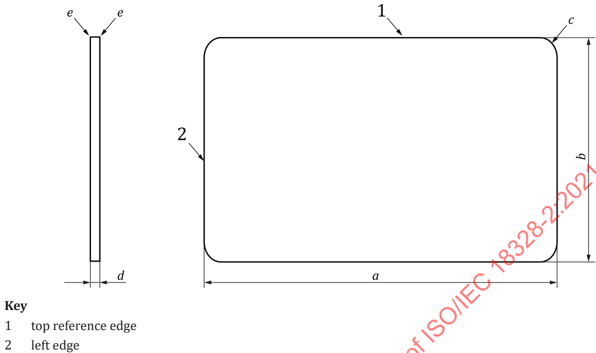
Figure A.1 — ID-T size card dimensions
