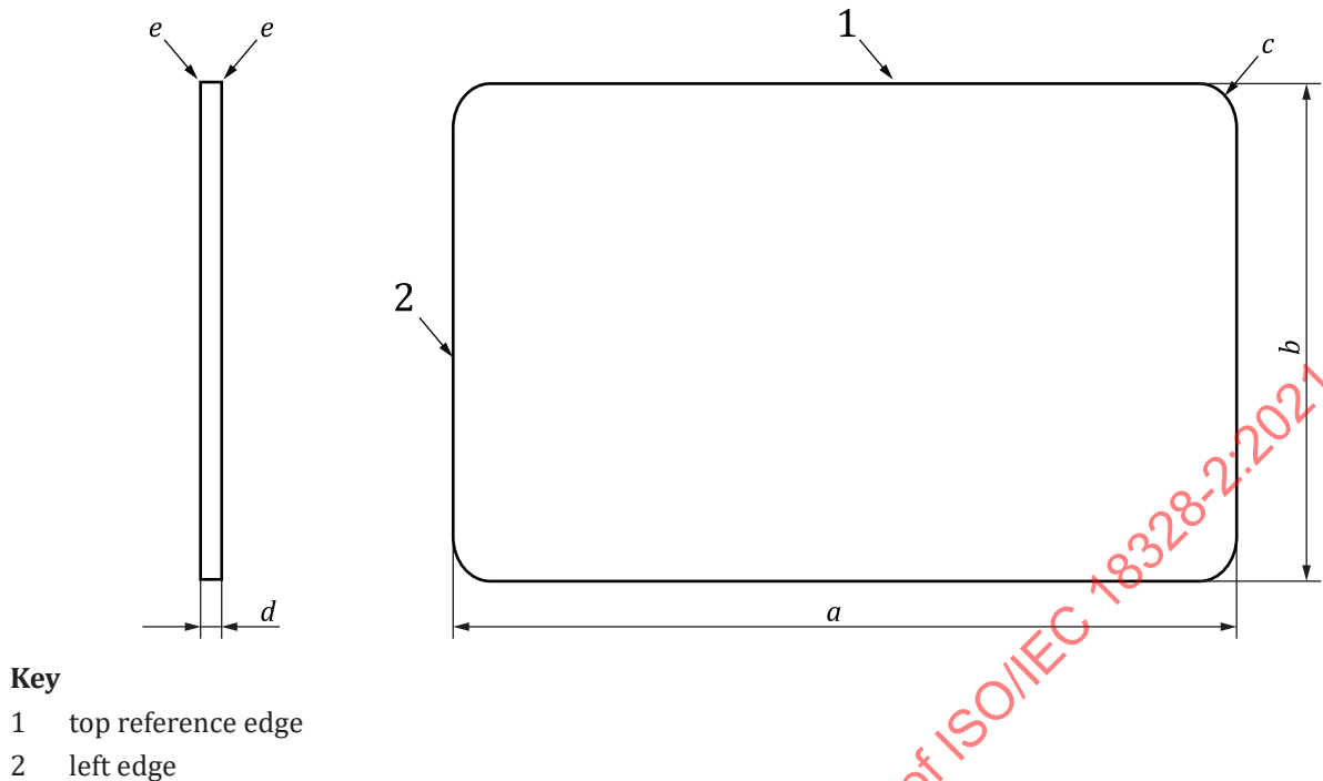
Figure B.1 — ID-B size card dimensions
