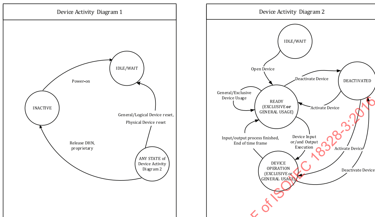
Figure 2 — State diagram of electronic device activities
