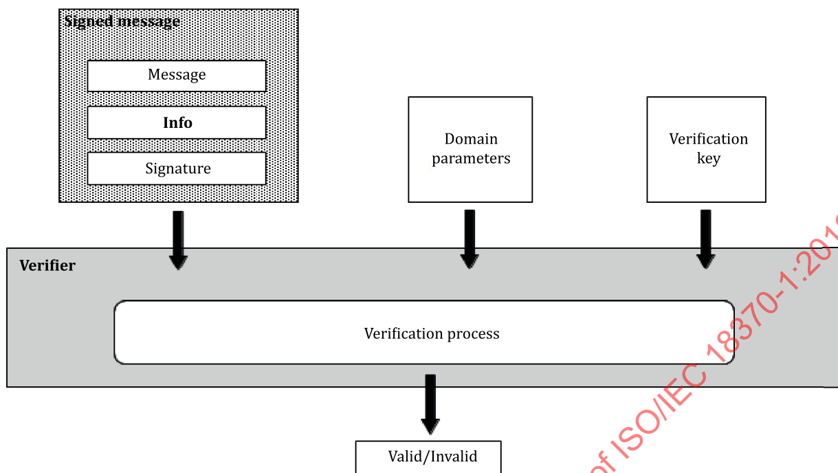
Figure 4 — Verification process
