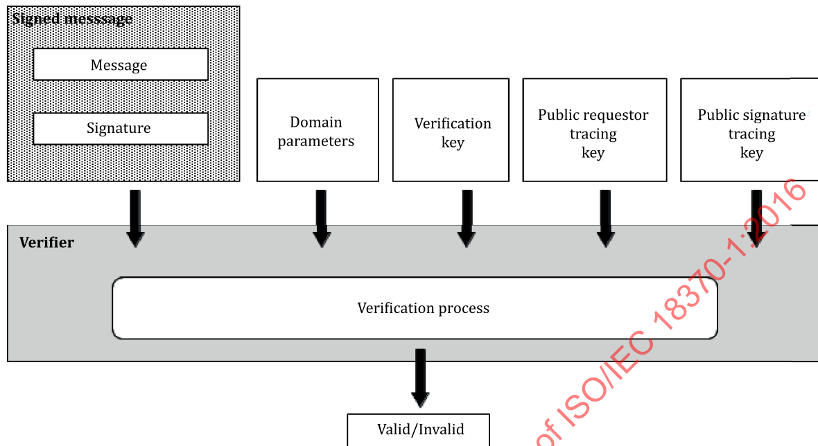
Figure 9 — Verification process
