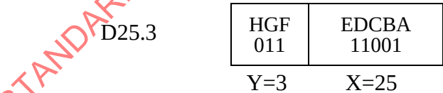
Figure 4-1. Character Notation Example (D25.3)
