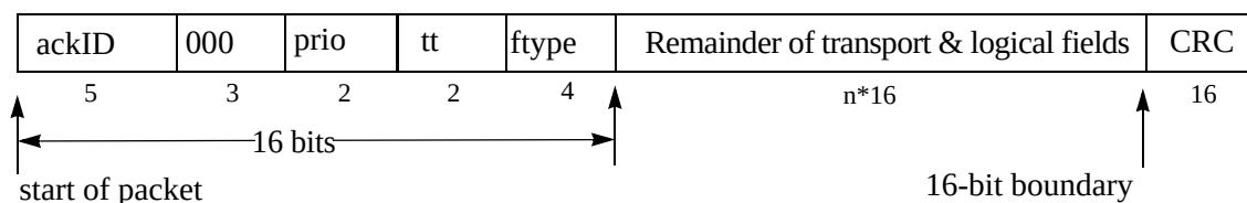
Figure 2-2. Packet Alignment
