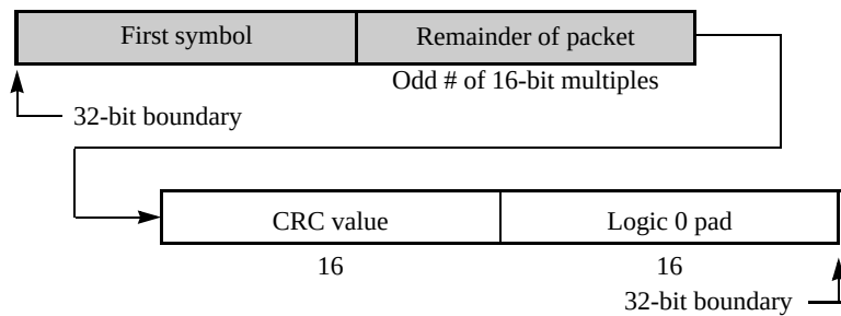
Figure 1-11. Padded Aligned Packet Bit Stream Example 1
