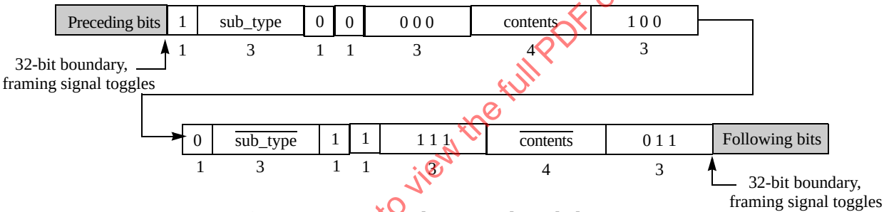
Figure 3-4. Type 4 Packet Control Symbol Format
