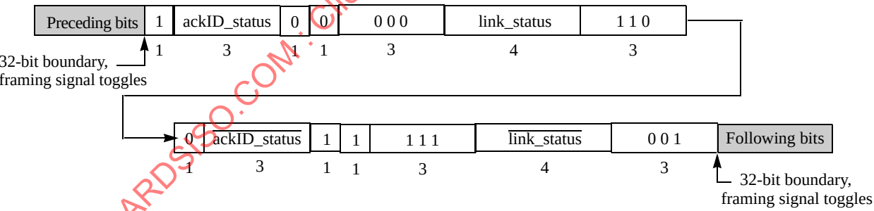
Figure 3-6. Type 6 Link-Response Control Symbol Format
