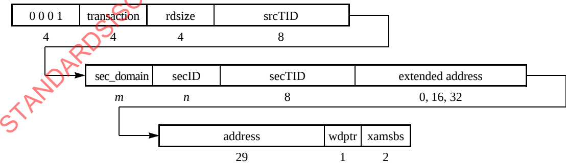
Figure 4-1. Type 1 Packet Bit Stream Format
