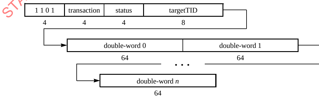
Figure 4-4. Type 13 Packet Bit Stream Format
