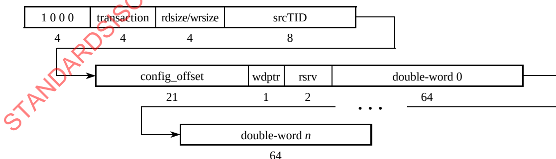
Figure 3-4. Type 8 Request Packet Bit Stream Format
