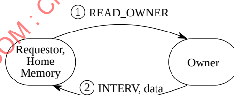
Figure 3-3. Read Operation to Local Modified Coherence Granule
