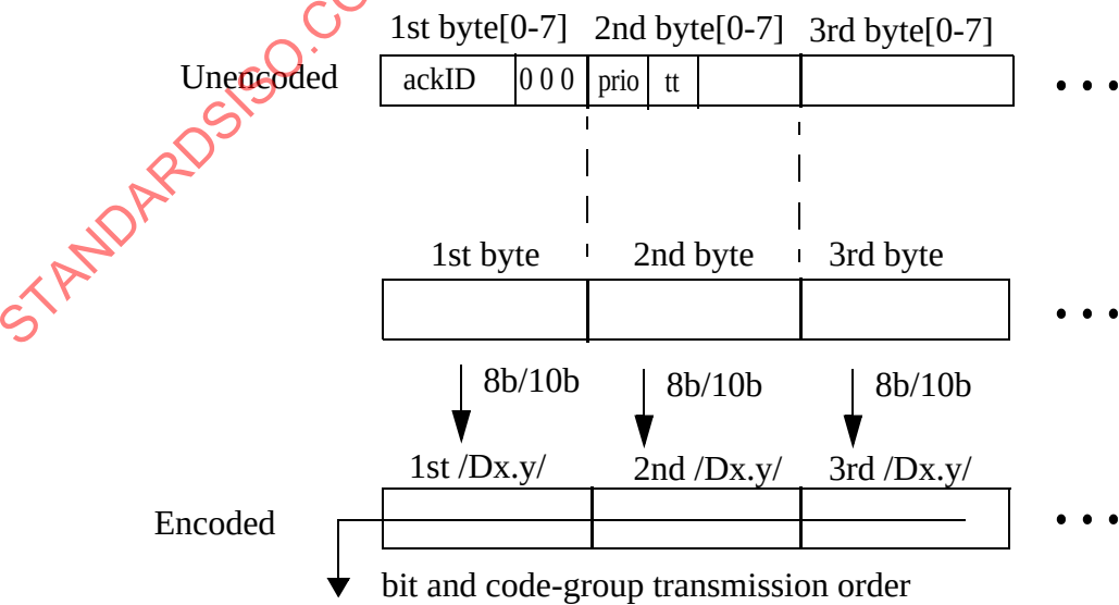
Figure 4-6. 1x Mode Packet Encoding and Transmission Order
