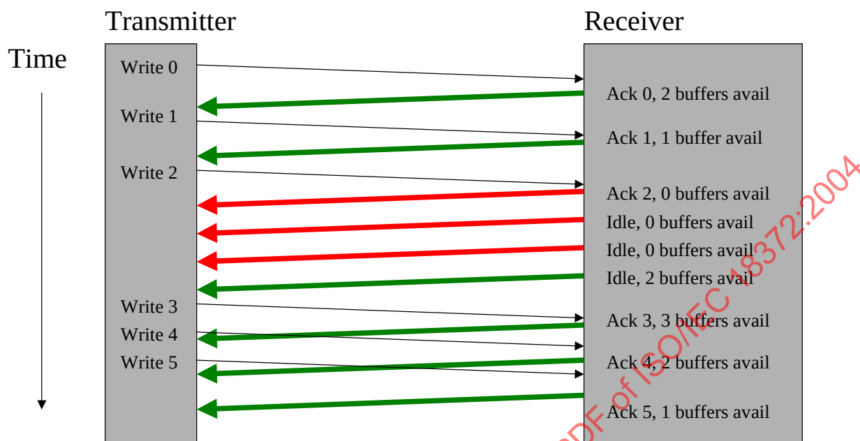
Figure 1-6. Transmitter-Controlled Flow Control
