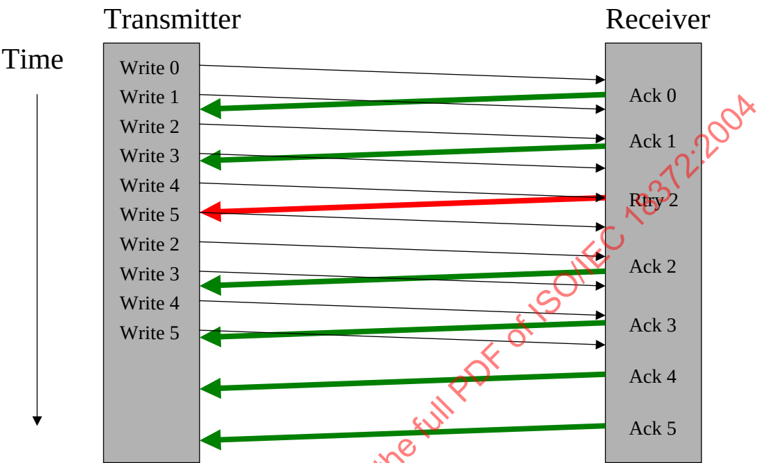
Figure 5-2. Receiver-Controlled Flow Control
