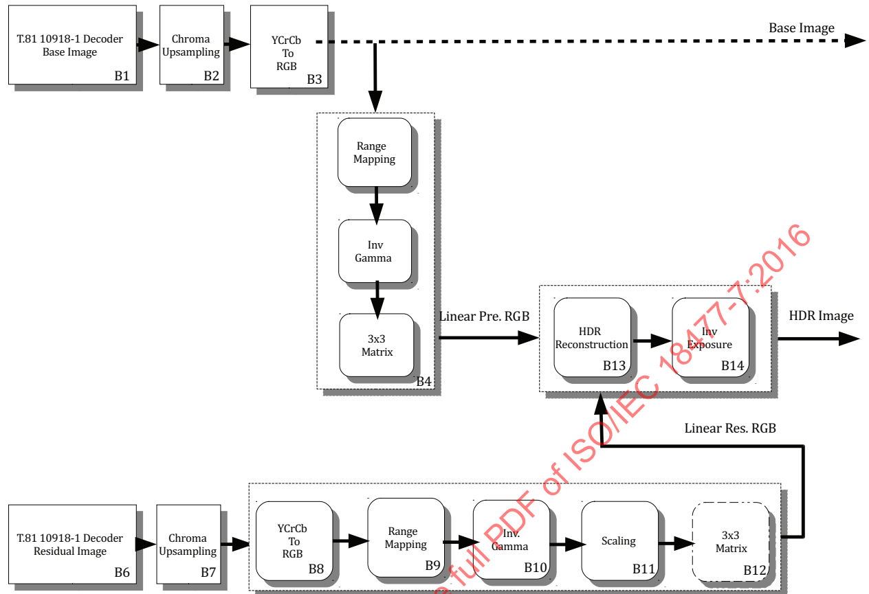
Figure E.2 — High level overview of the decoding process of a profile B compliant decoder
