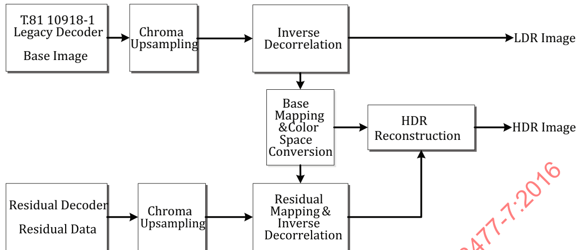
Figure 1 — Overview on the decoding process
