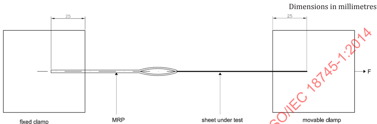
Figure 13 — Sheet Pull Apparatus
