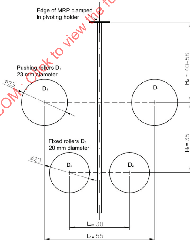
Figure 8 — Apparatus to impose cyclic motion
