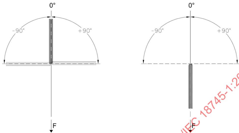
Figure 12 — Sheet Bending Illustration
