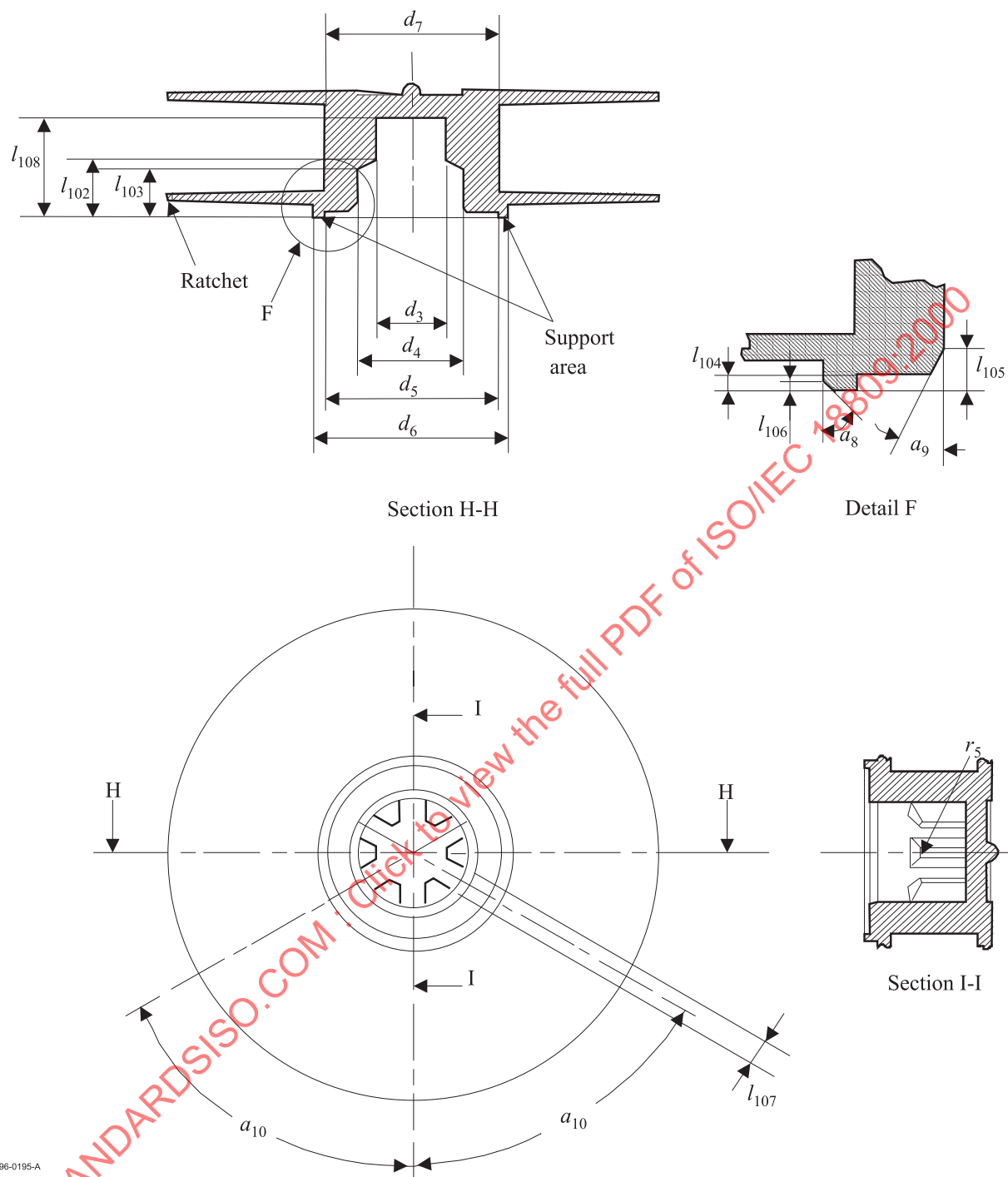
Figure 22 - Cartridge reel
