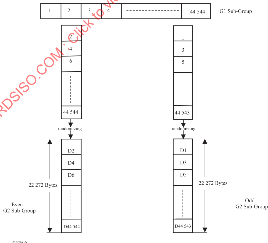
Figure 33 - G2 Sub-Groups
