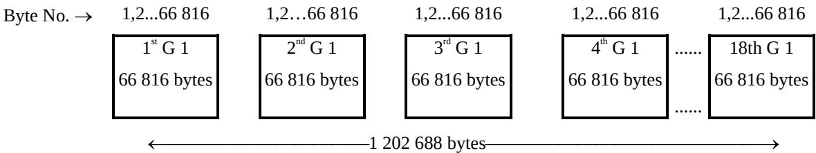
Figure 32 - G1 Sub-Groups
