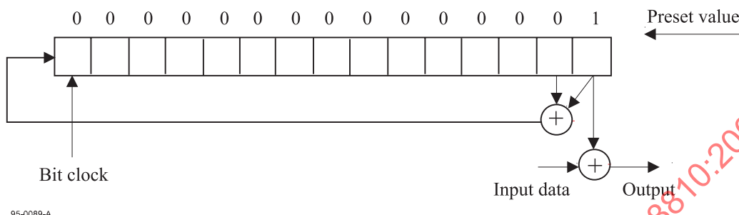
Figure 33 - Shift register
