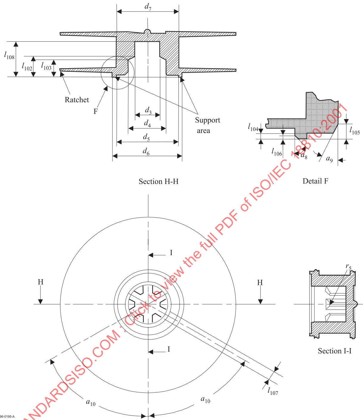
Figure 22 - Cartridge reel
