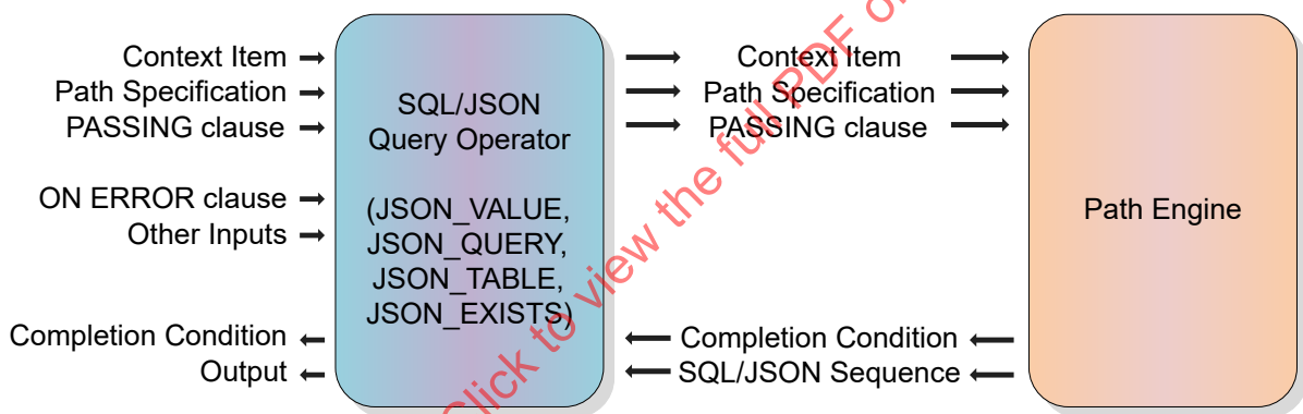
Figure 2 — The SQL/JSON path language architecture
