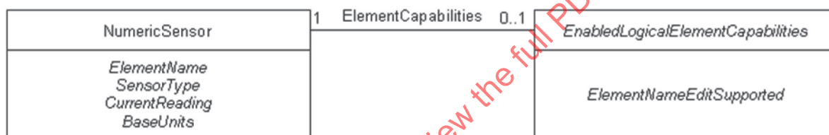
Figure 5 — class: CIM_NumericSensor
