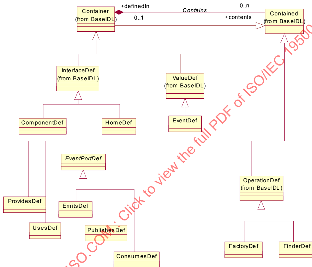
Figure 11.13- Containment Hierarchy
