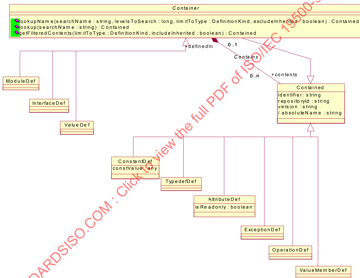
Figure 11.4- Containment Hierarchy
