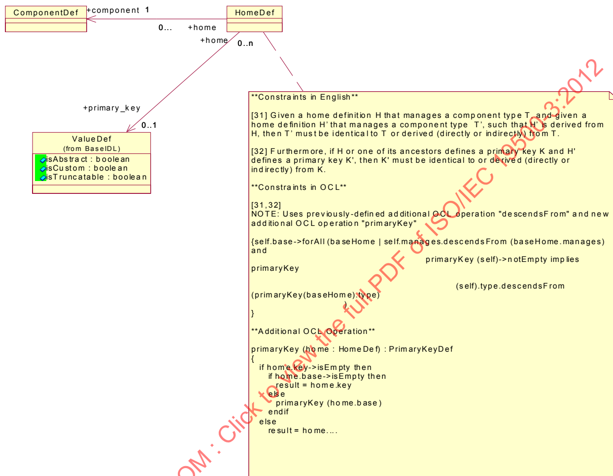
Figure 11.19- Home and Primary Key Constraints
