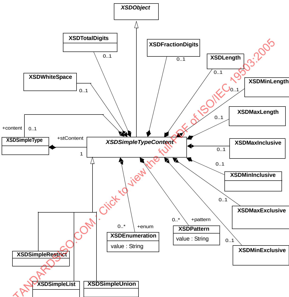
Figure 8.5 - XML Schema Simple type content declarations
