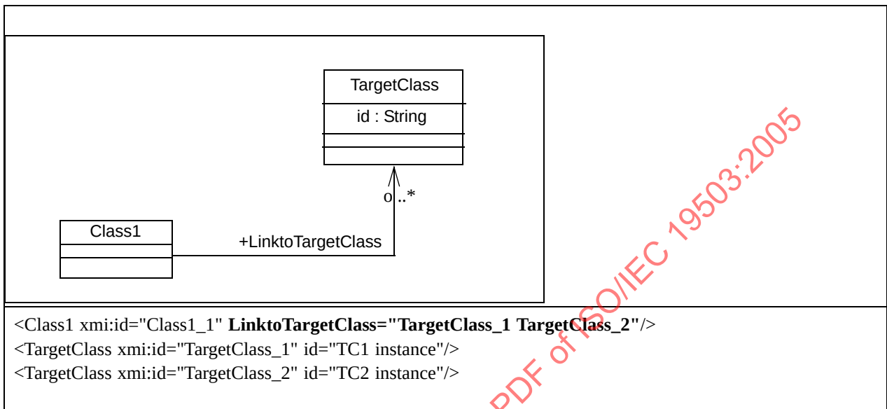
Example 6.6 - Association from an instance of a class to instances of another class
