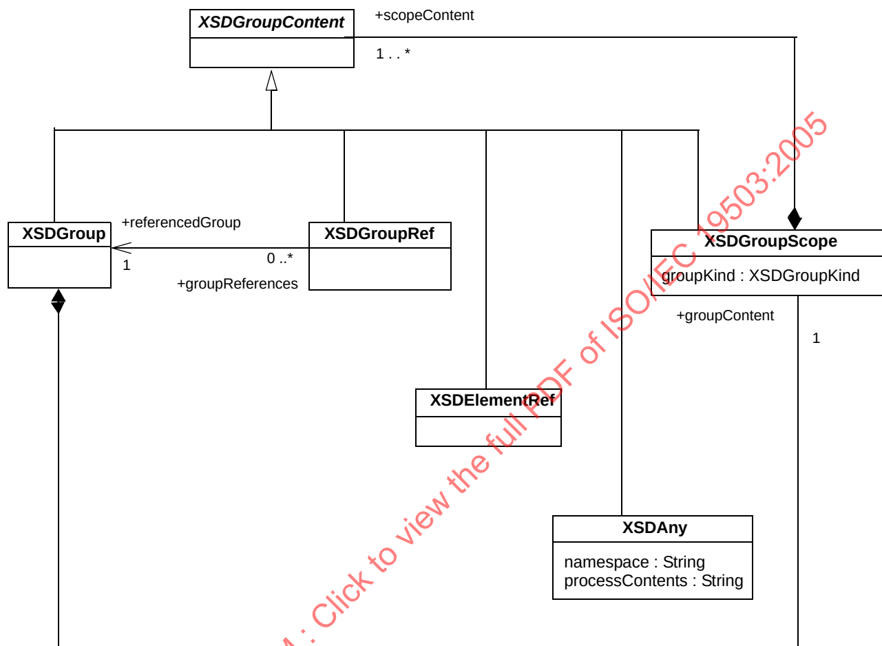
Figure 8.9 - XML Schema group declarations
