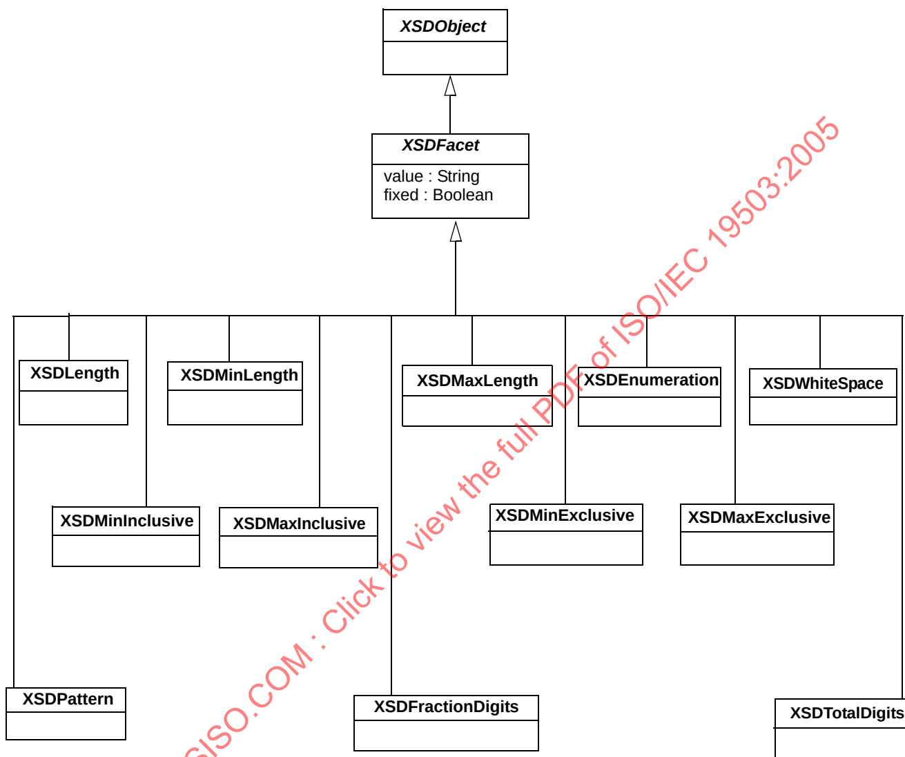
Figure 8.6 - XML Schema Facets
