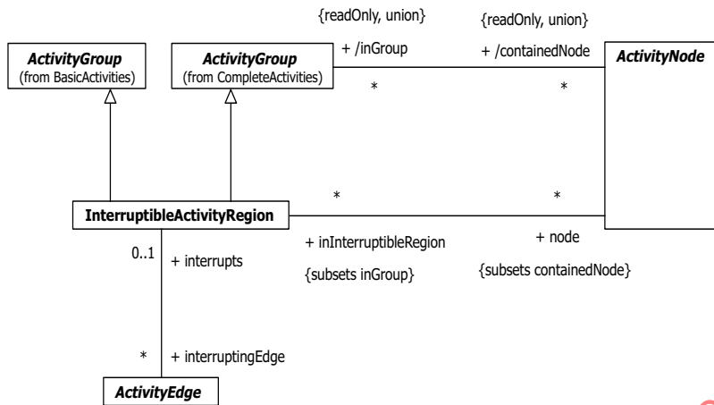
Figure 12.20 - Interruptible regions
