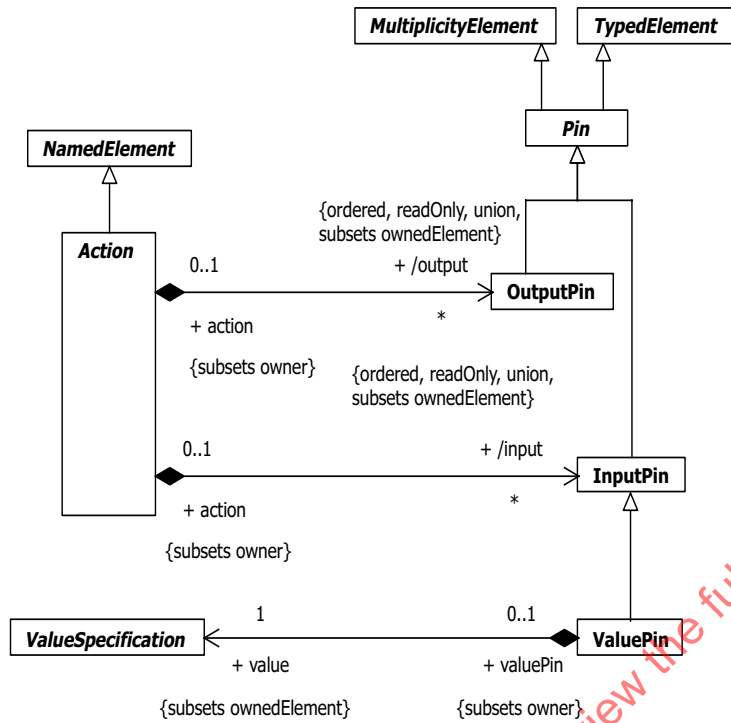
Figure 11.3 - Basic pins
