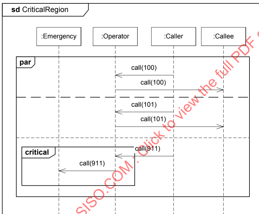
Figure 14.9 - Critical Region
