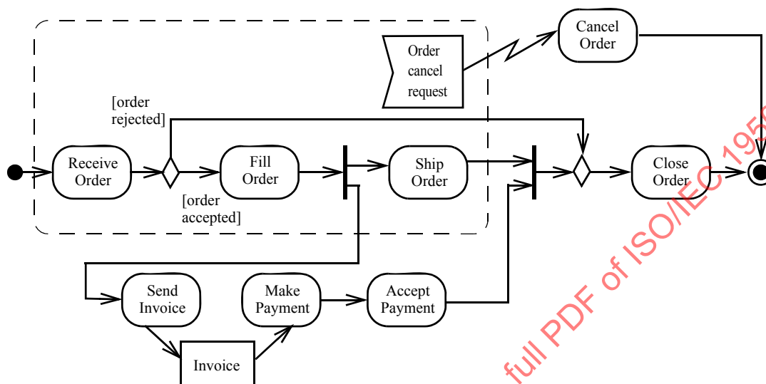
Figure 12.100 - InterruptibleActivityRegion example
