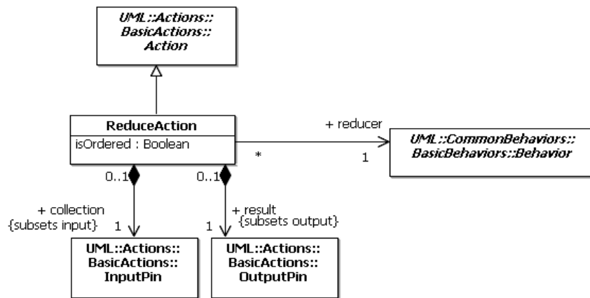
Figure 11.17 - ReduceAction (CompleteActions)
