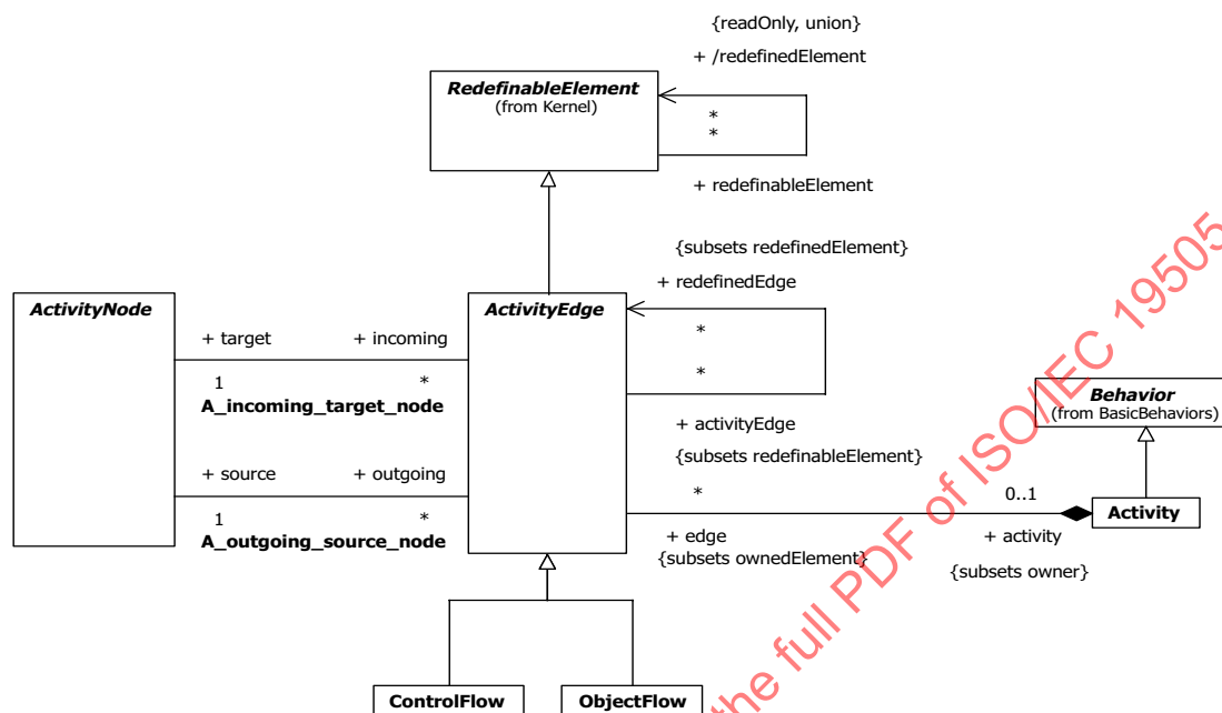
Figure 12.5 - Flows
