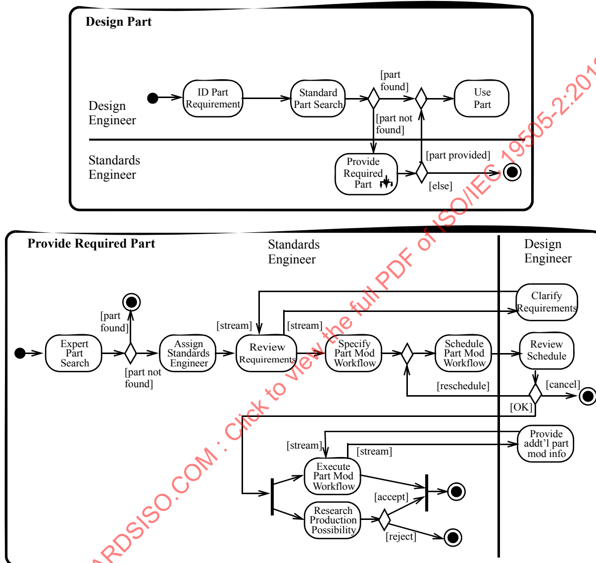
Figure 12.36 - Workflow example
