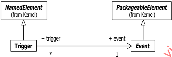
Figure 13.11 - Triggers
