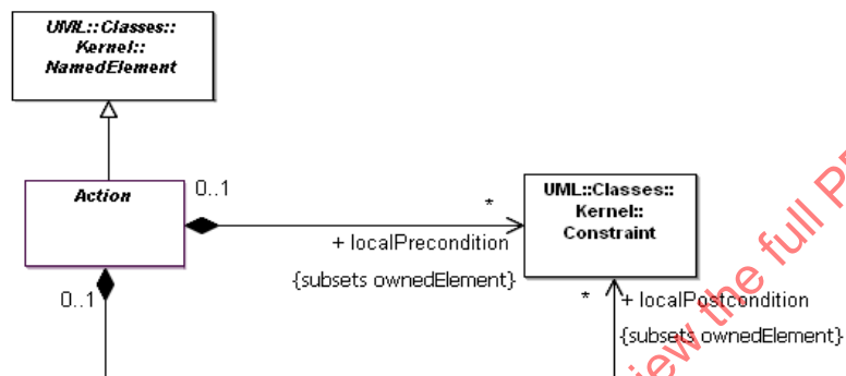
Figure 12.13 - Constraints (CompleteActivities)
