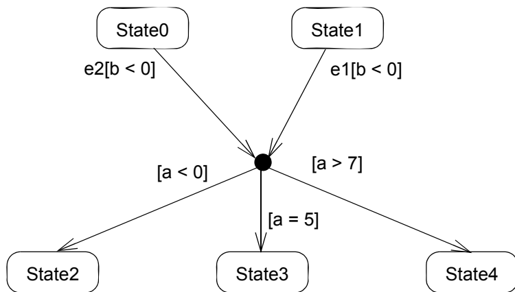
Figure 15.22 - Junction
