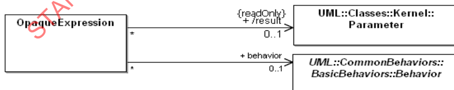
Figure 13.7 - Expression
