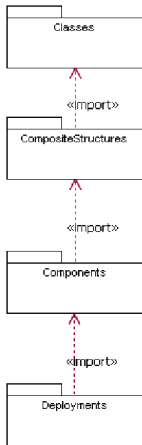
Figure 6.3 - UML packages that support structural modeling
