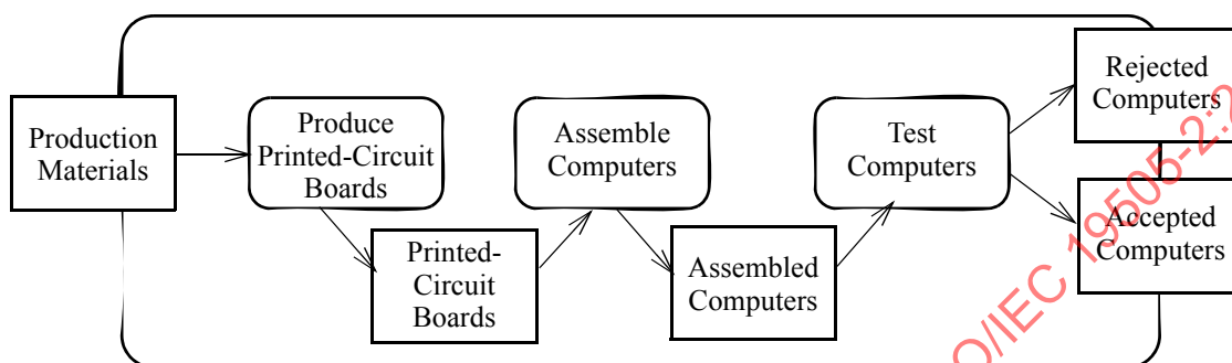
Figure 12.55 - Example of activity parameter nodes
