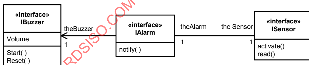
Figure 7.59 - A set of collaborating interfaces
