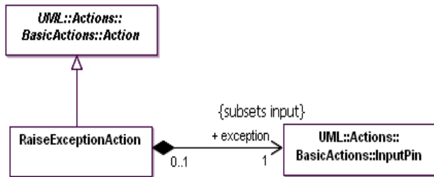
Figure 11.19 - Raise exception action
