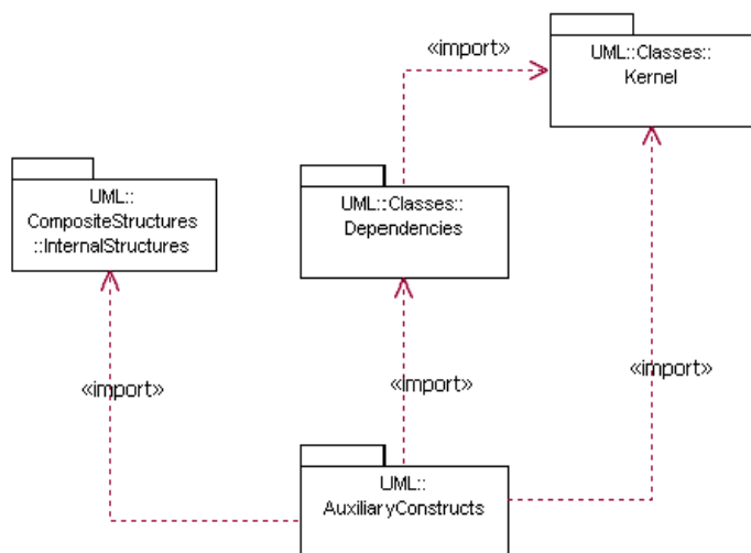
Figure 6.5 - UML packages that support auxiliary constructs
