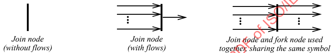
Figure 12.101 - Join node notations
