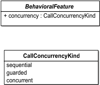
Figure 13.10 - Extensions to behavioral features
