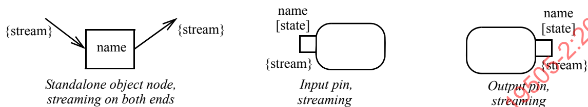
Figure 12.121 - Stream pin notations
