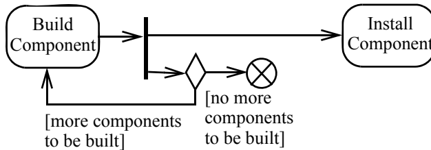
Figure 12.93 - Flow final example without merge edge
