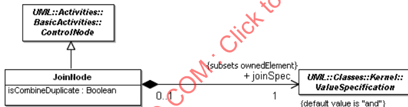
Figure 12.19 - Control nodes (CompleteActivities)
