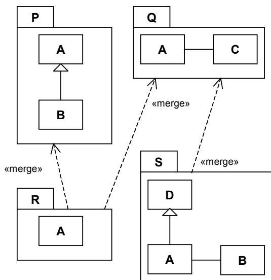
Figure 7.68 - Simple example of package merges
