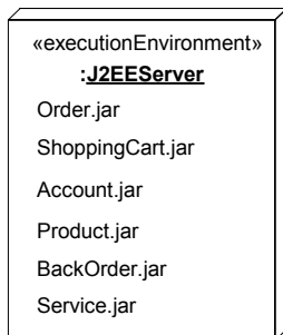
Figure 10.15 - Notation for an ExecutionEnvironment (example of an instance of a J2EEServer ExecutionEnvironment)
