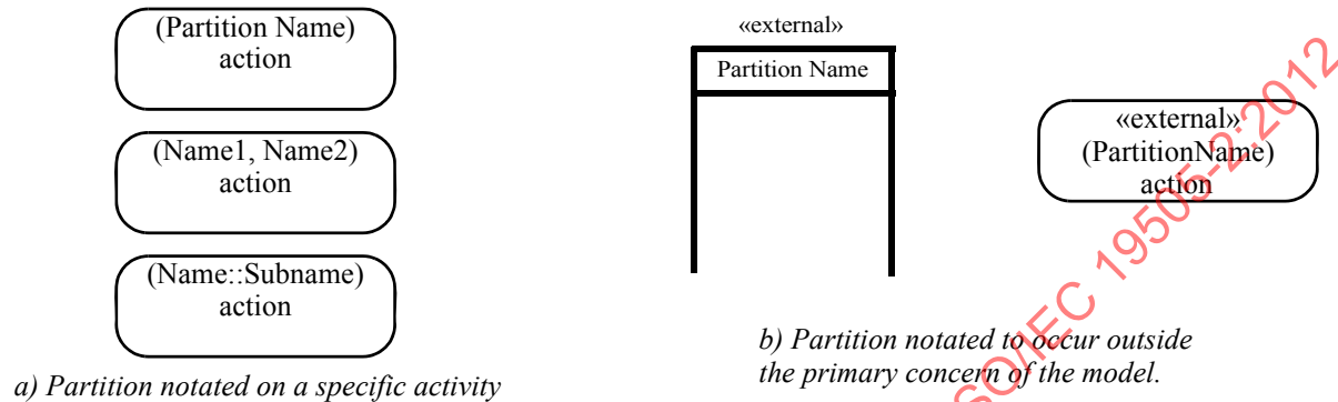
Figure 12.58 - Activity partition notations
