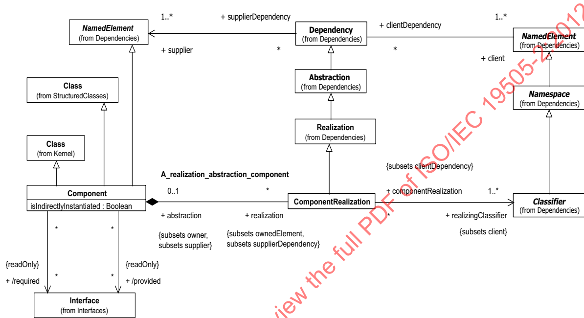
Figure 8.2 - The metaclasses that define the basic Component construct
