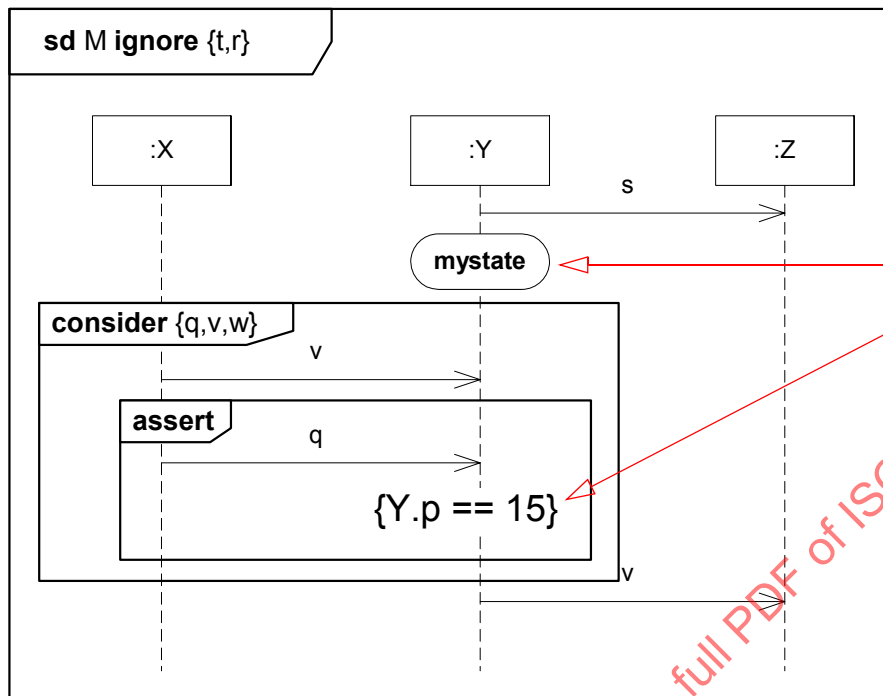
Figure 14.24 - Ignore, Consider, assert with State Invariants
