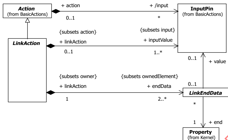
Figure 11.8 - Link identification
