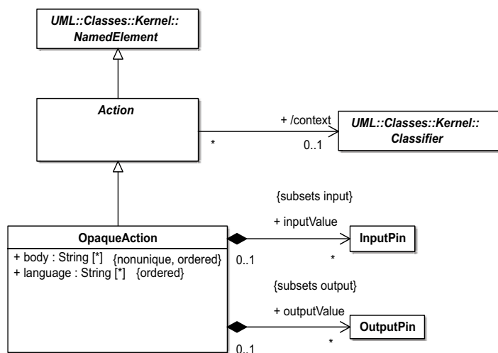
Figure 11.2 - Basic Actions
