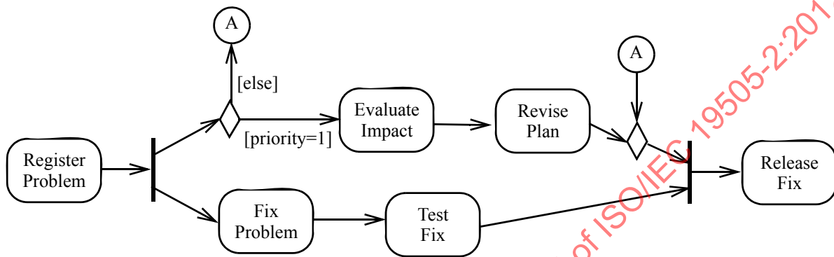
Figure 12.43 - Connector example
