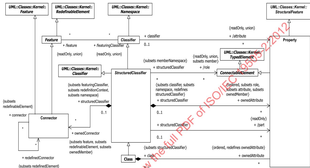
Figure 9.2 - Structured classifier
