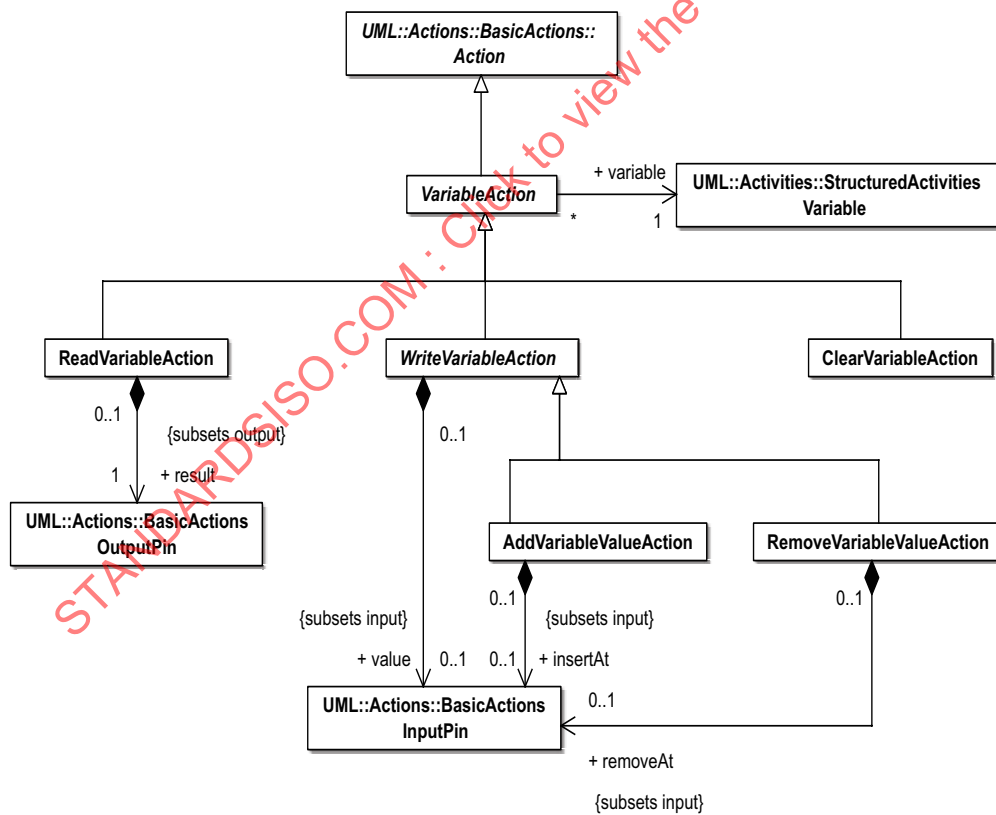
Figure 11.18 - Variable actions
