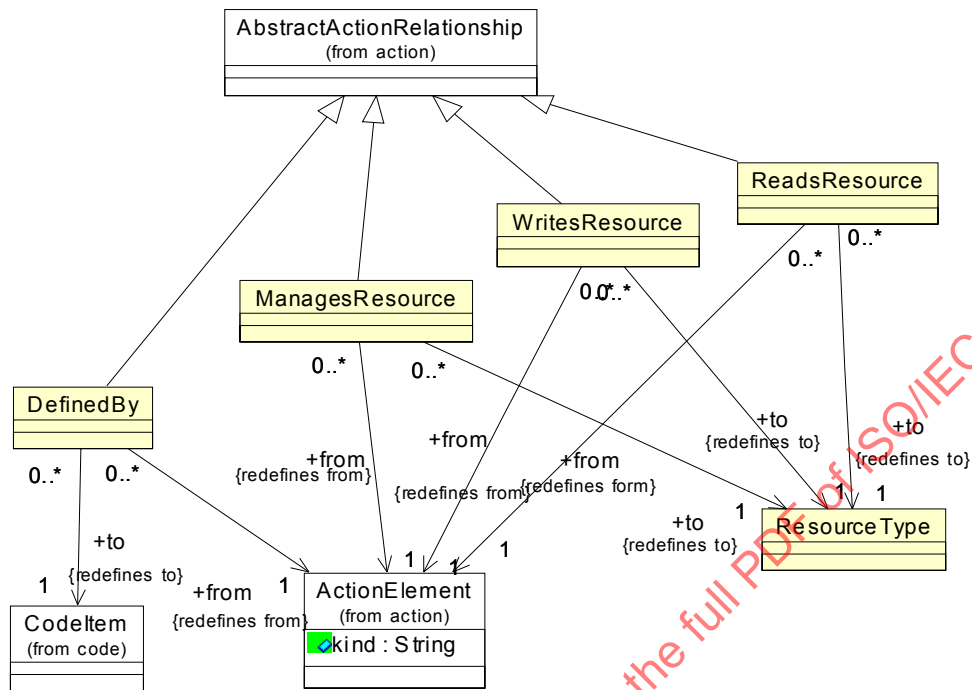
Figure 15.6 - PlatformActions Class Diagram
