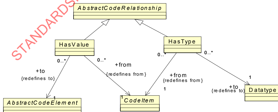
Figure 12.17 - TypeRelations Class Diagram
