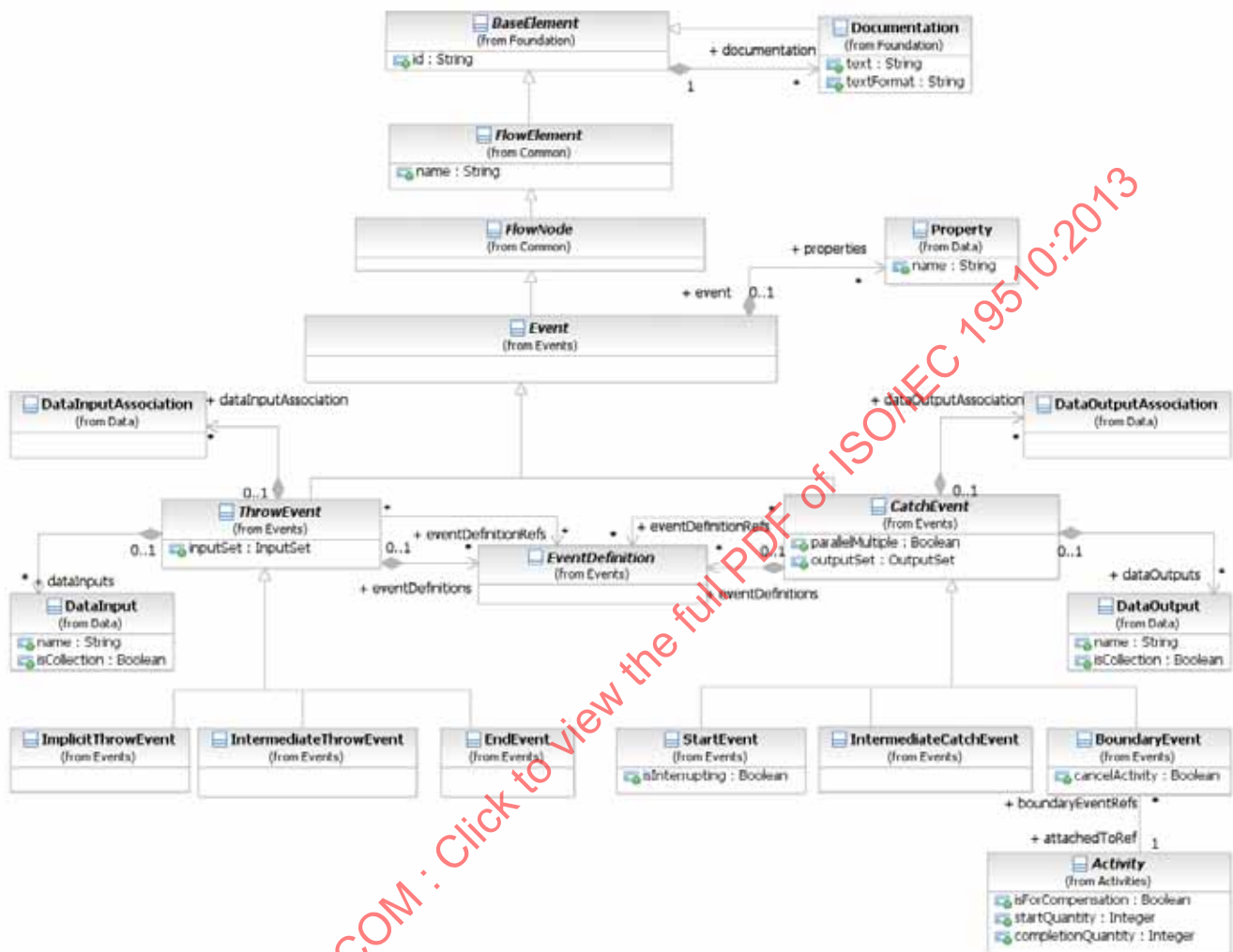
Figure 8.20 – Event class diagram
