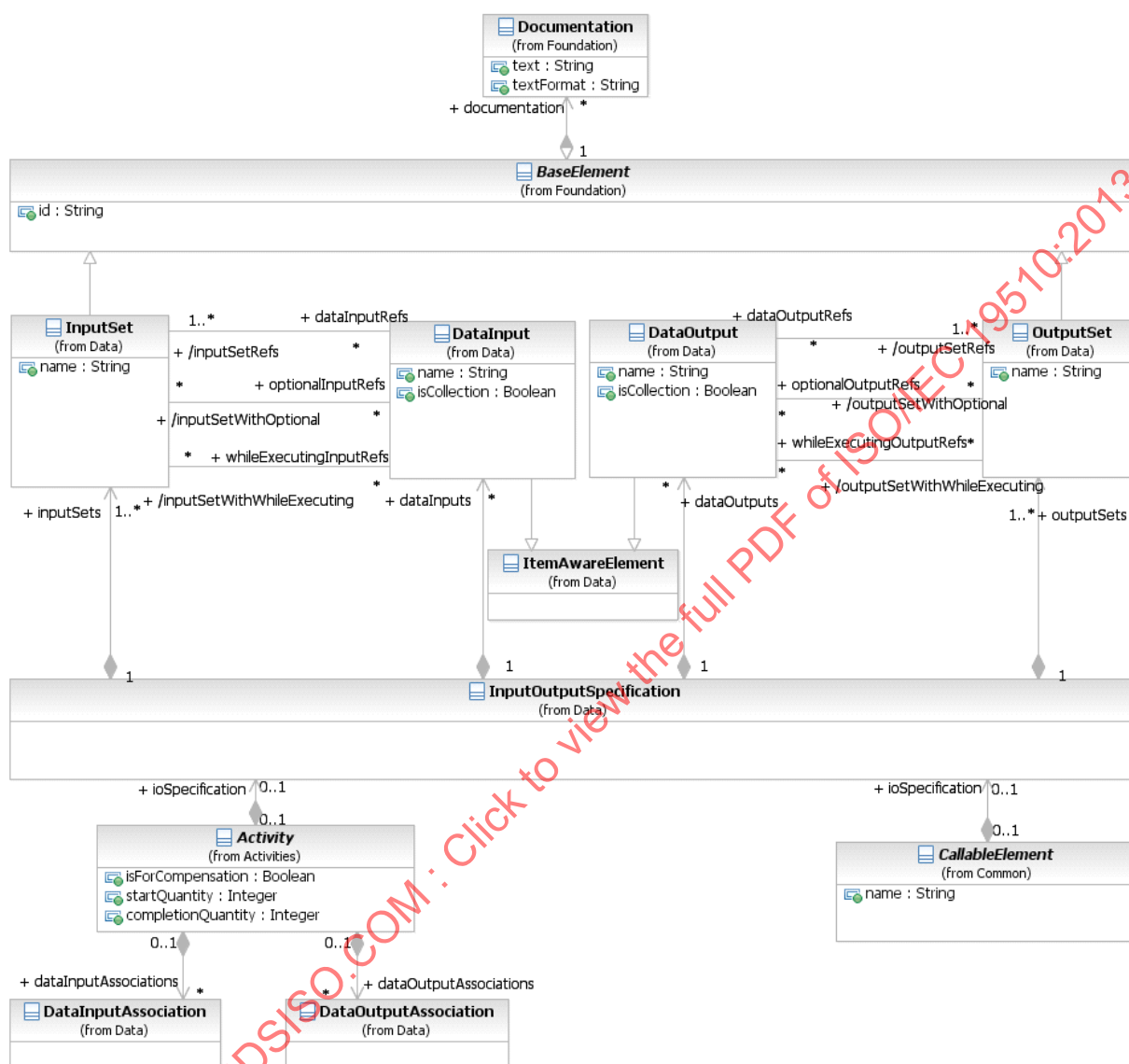
Figure 10.57 – InputOutputSpecification class diagram
