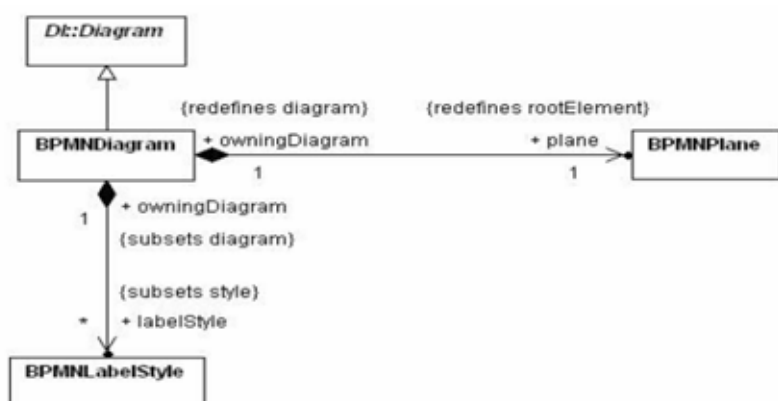
Figure 12.1 – BPMN Diagram
