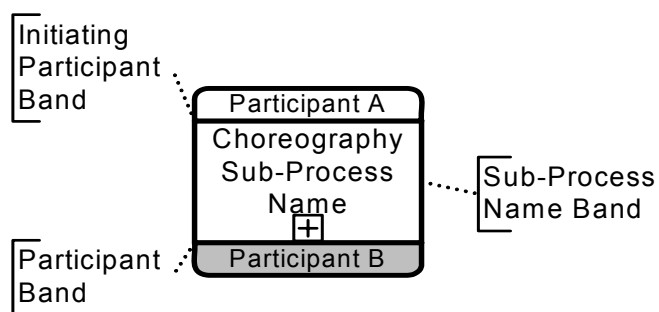
Figure 11.17– A Sub-Choreography
