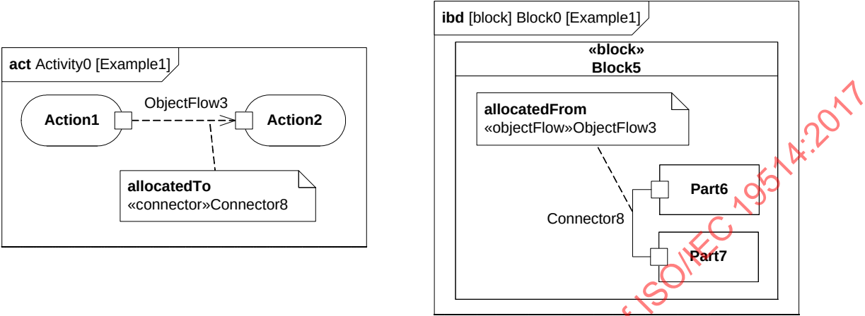
Figure 15.5 - Example of flow allocation from ObjectFlow to Connector
