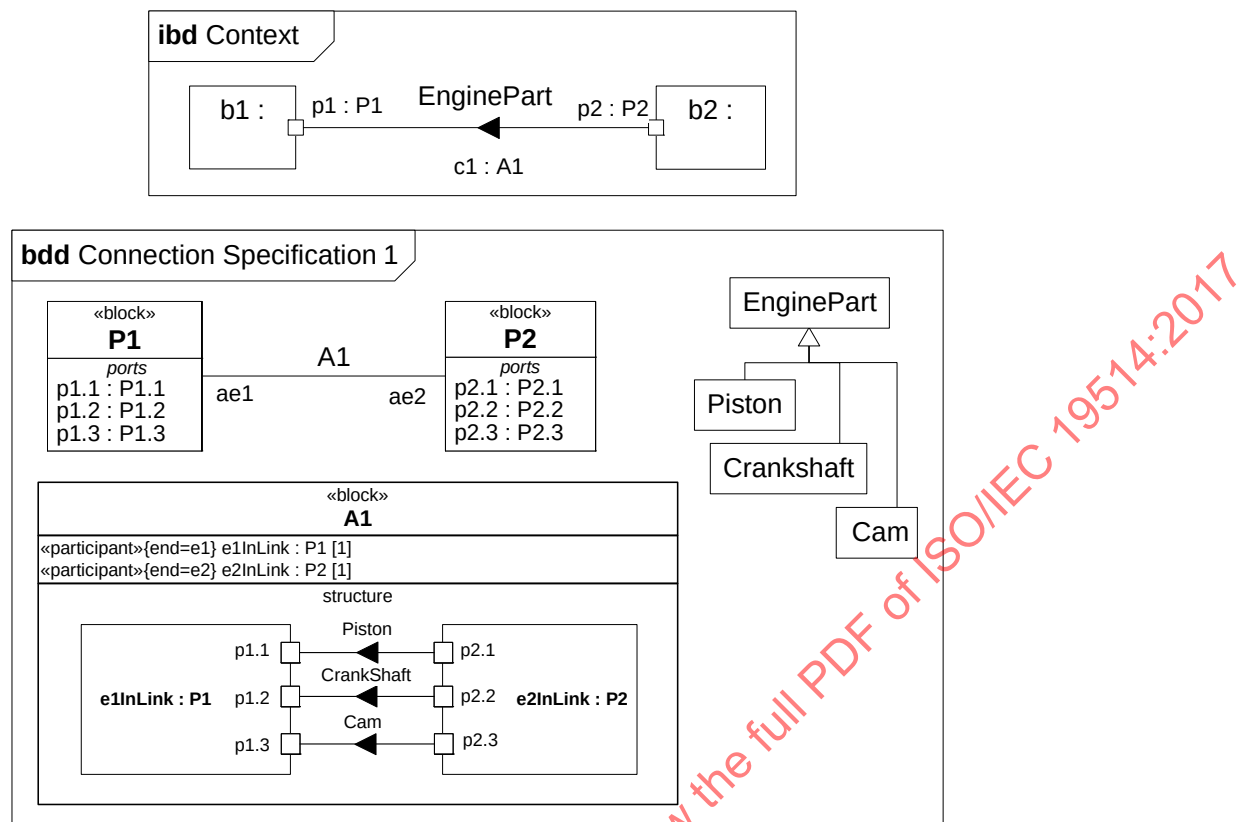
Figure 9.16 - Usage example of item flow decomposition
