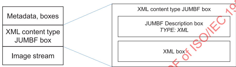
Figure B.9 — Generated JUMBF box by encapsulating procedure
