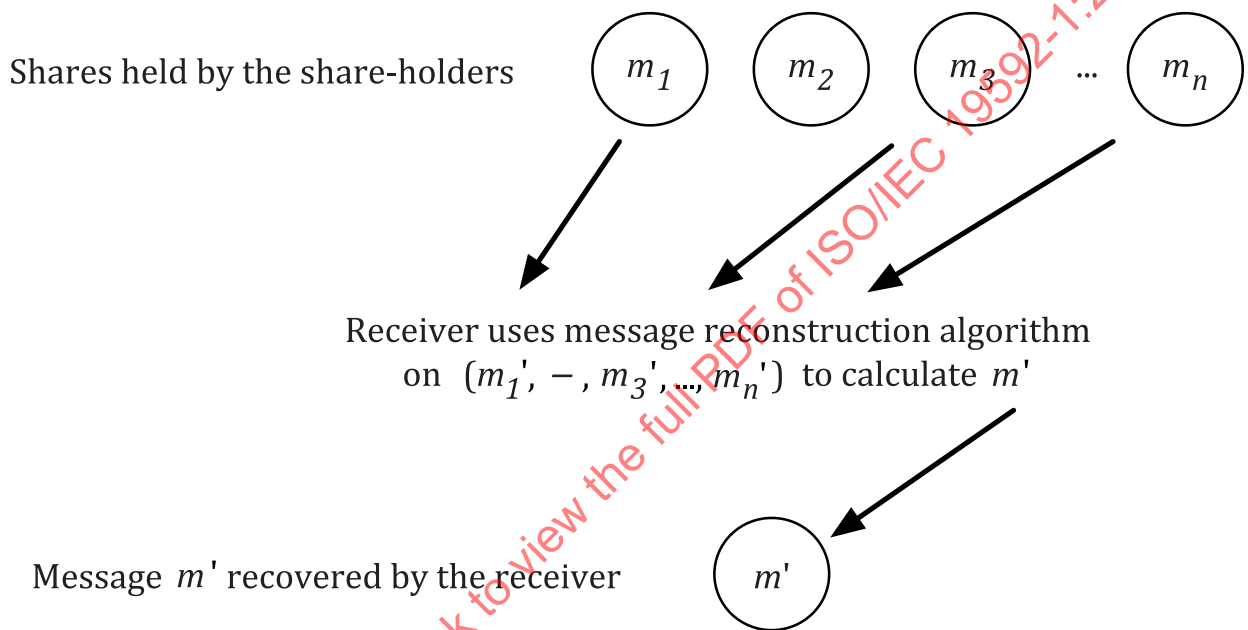
Figure 2 — Example of a message reconstruction process
