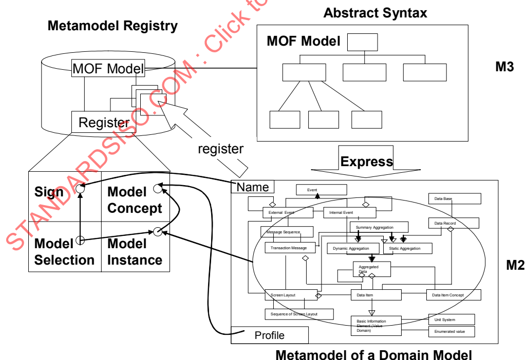
Figure 14 — Registration of metamodels as an upper model
