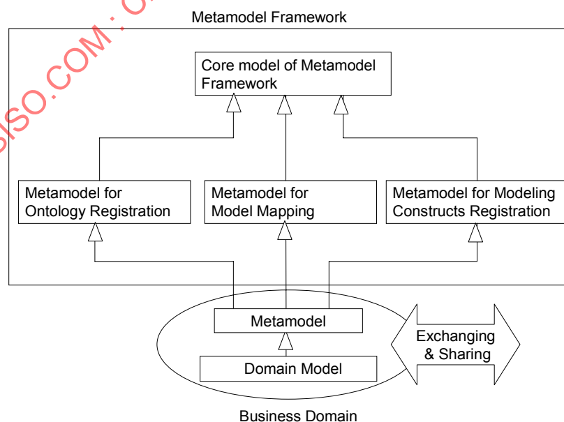
Figure 5 — Metamodel framework architecture
