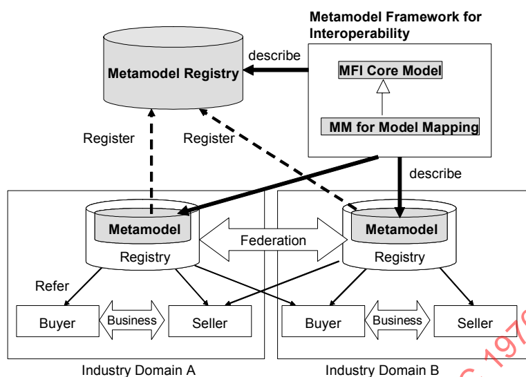
Figure 4 — Registry federation by the metamodel frameworks
