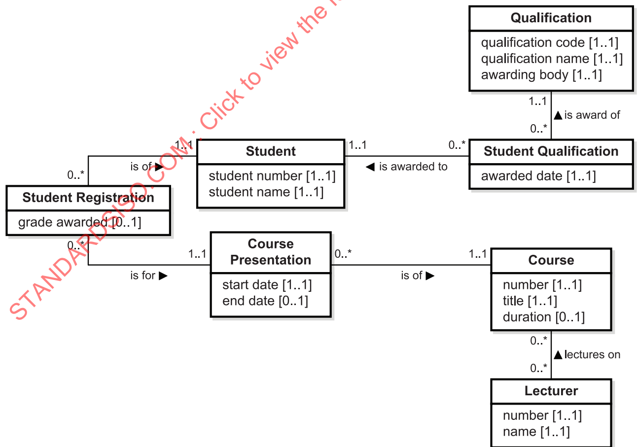
Figure C.1 — UML class diagram for the student registration scenario
