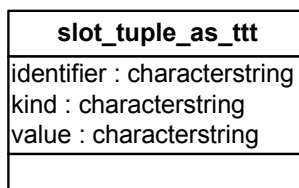
Figure 7 — UML presentation of slot_tuple_as_ttt datatype
