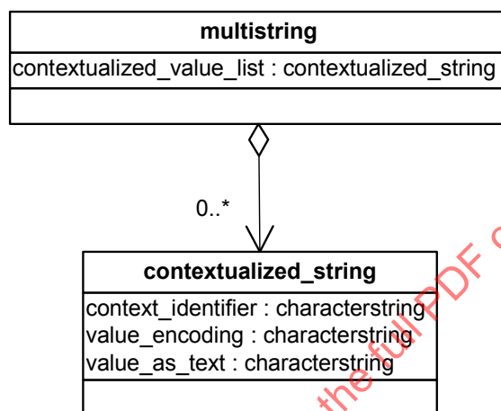
Figure 4 — UML presentation of: multistring, contextualized_string
