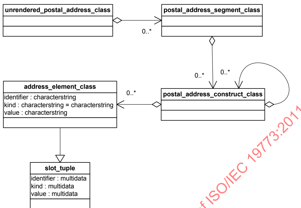
Figure 18 — UML presentation of the classes: unrendered postal address, postal address segment, postal address construct, address element.
