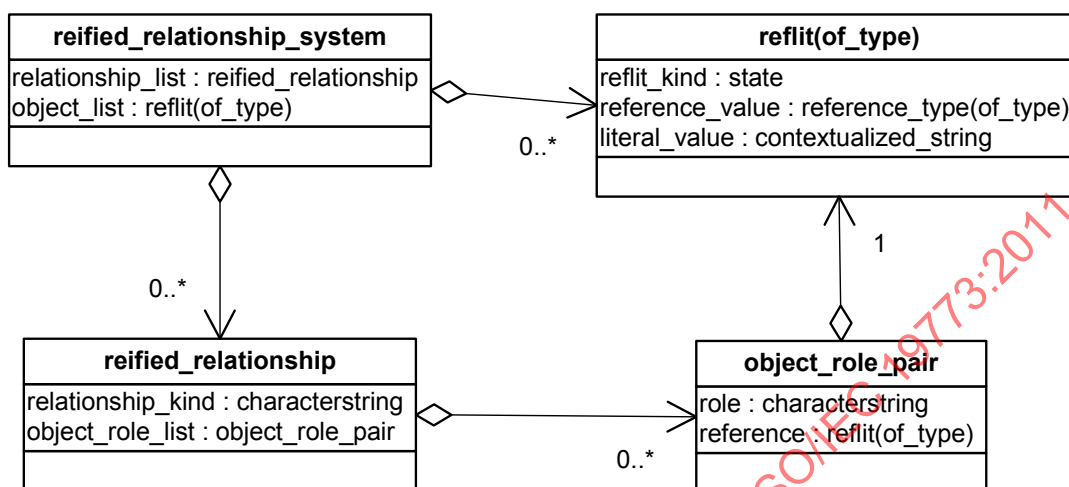
Figure 14 — UML presentation of Reified Relationship Systems
