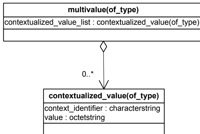
Figure 2 — UML presentation of: multivalue , contextualized_value
