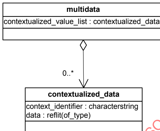
Figure 3 — UML presentation of: multidata , contextualized_data
