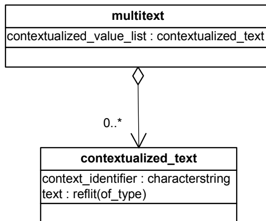
Figure 5 — UML presentation of: multitext, contextualized_text
