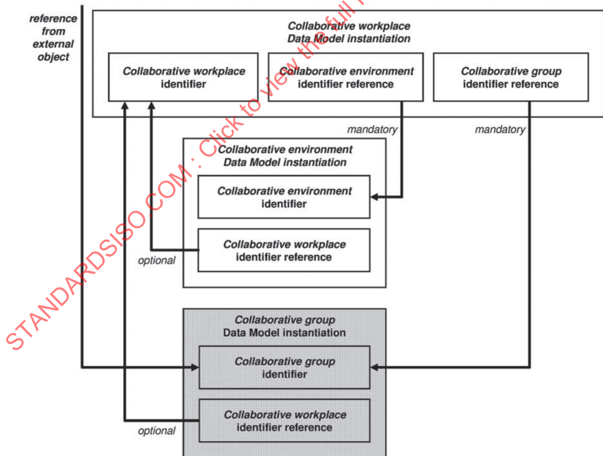
Figure 3 — Linkages between the collaborative group , the associated collaborative workplace , and the associated collaborative environment
