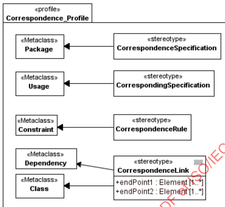
Figure 40 – Graphical representation of the UML profile for correspondences specifications
