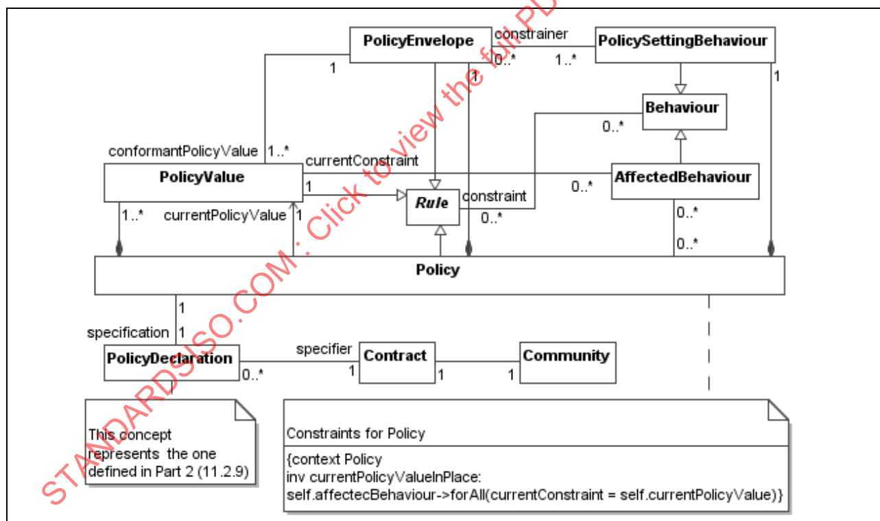
Figure 6 – Policy concepts
