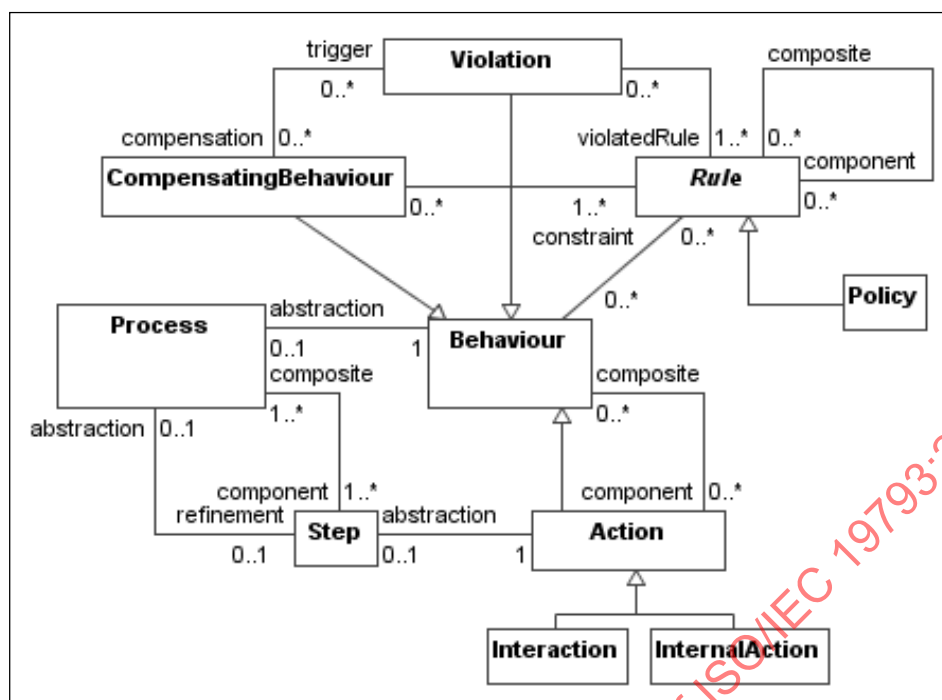
Figure 5 – Behaviour concepts
