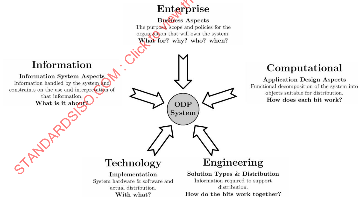
Figure 1 – RM-ODP viewpoints
