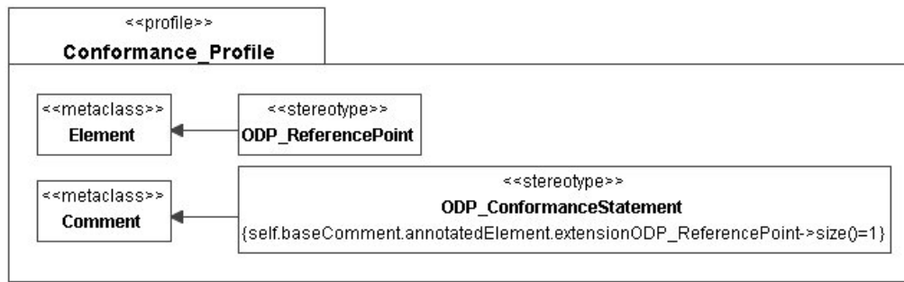
Figure 41 – UML profile for conformance
