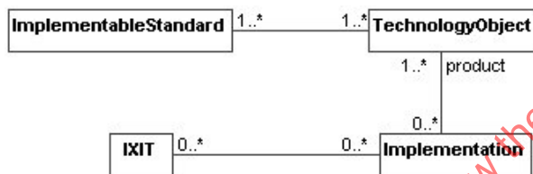
Figure 37 – Model of the technology language
