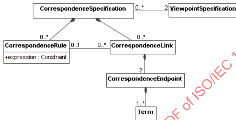
Figure 39 – Correspondences specification concepts
