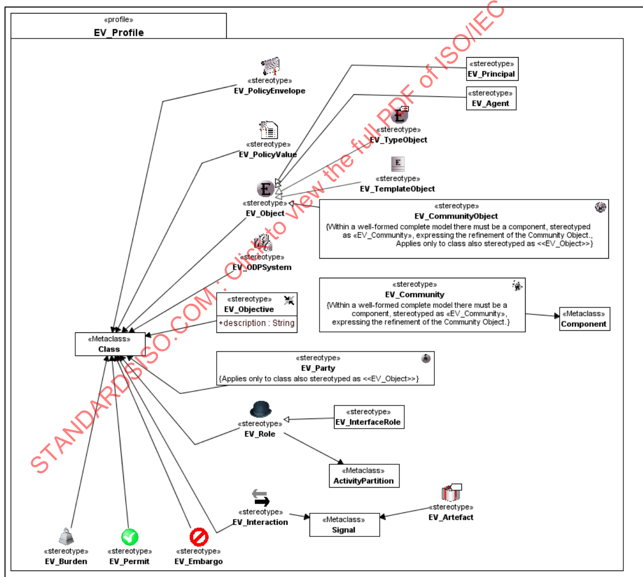
Figure 12 – Classifiers
