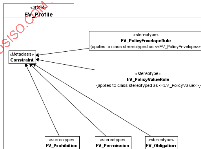
Figure 14 – Constraints
