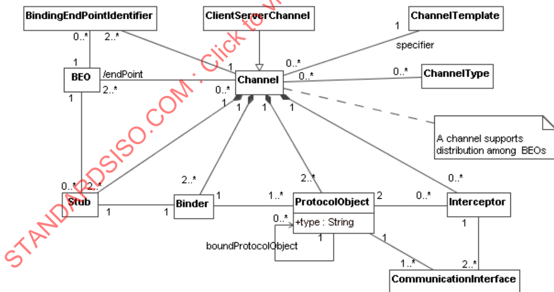
Figure 30 – Engineering language model – channels
