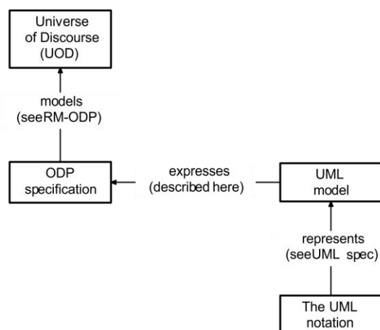
Figure 2 – Relationships between UOD, ODP specifications, and UML models
