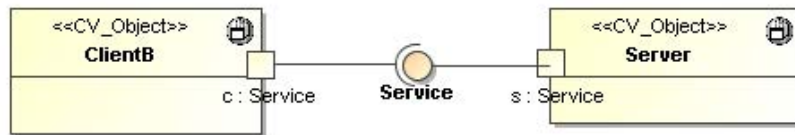
Figure 24 – An implicit primitive binding between two interfaces
