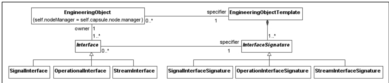
Figure 28 – Engineering interfaces
