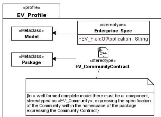
Figure 11 – Model management
