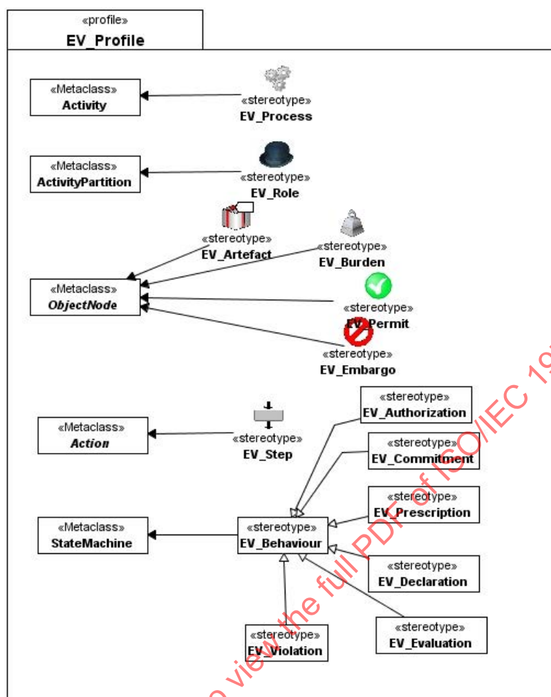
Figure 13 – Activities
