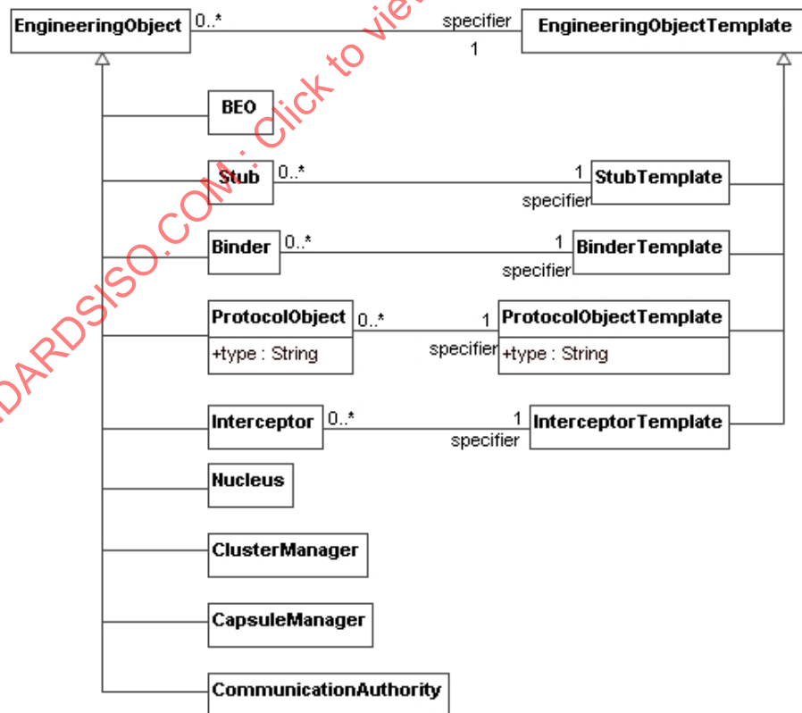
Figure 27 – Engineering objects
