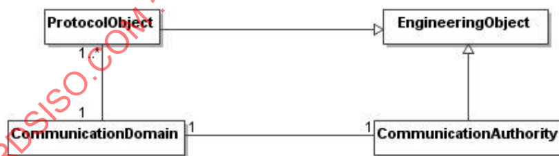
Figure 31 – Domains
