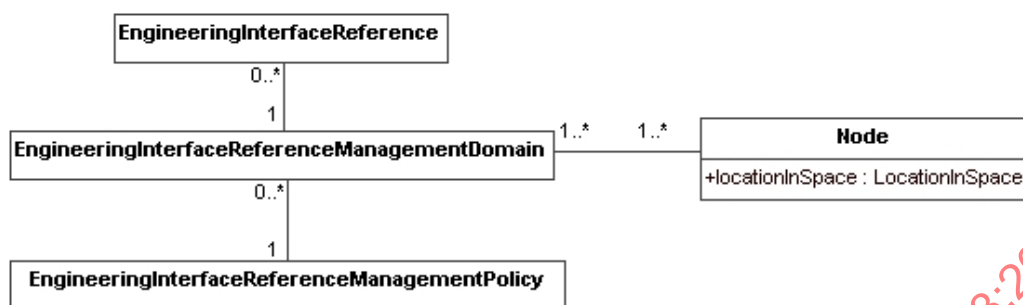
Figure 32 – Engineering language model – identifiers
