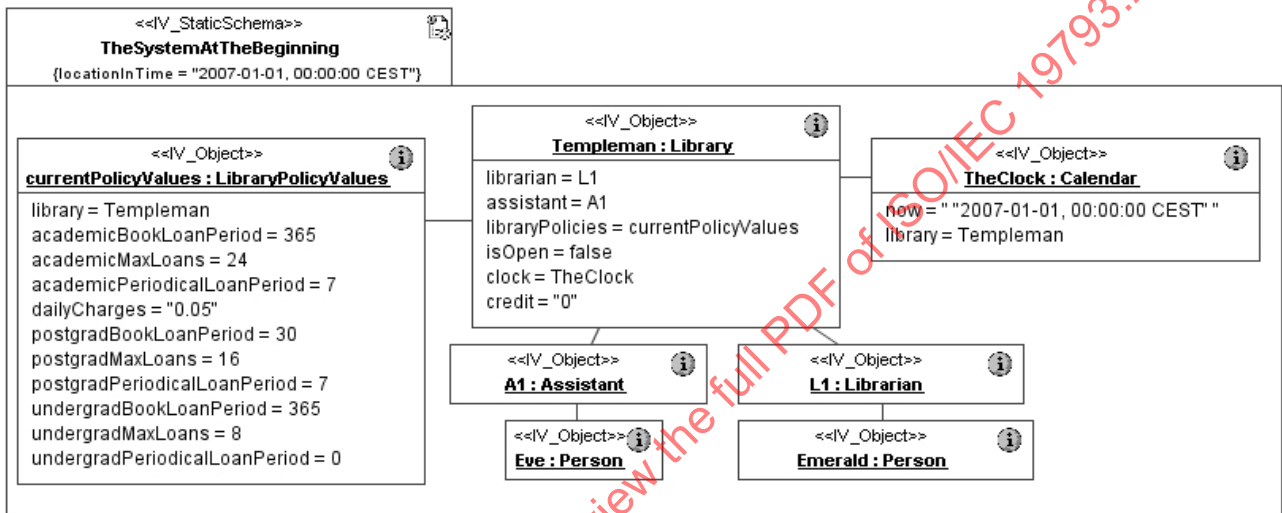
Figure A.22 – Static schema with the initial state of the Library system
