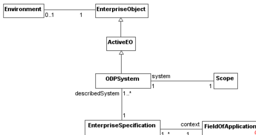
Figure 3 – System concepts
