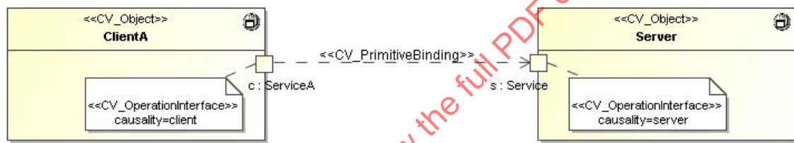
Figure 22 – An explicit primitive binding between two interfaces
