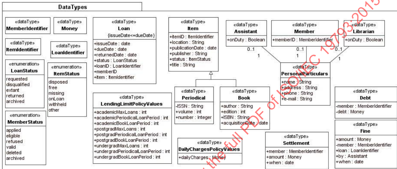
Figure A.32 – Data types handled by the computational objects
