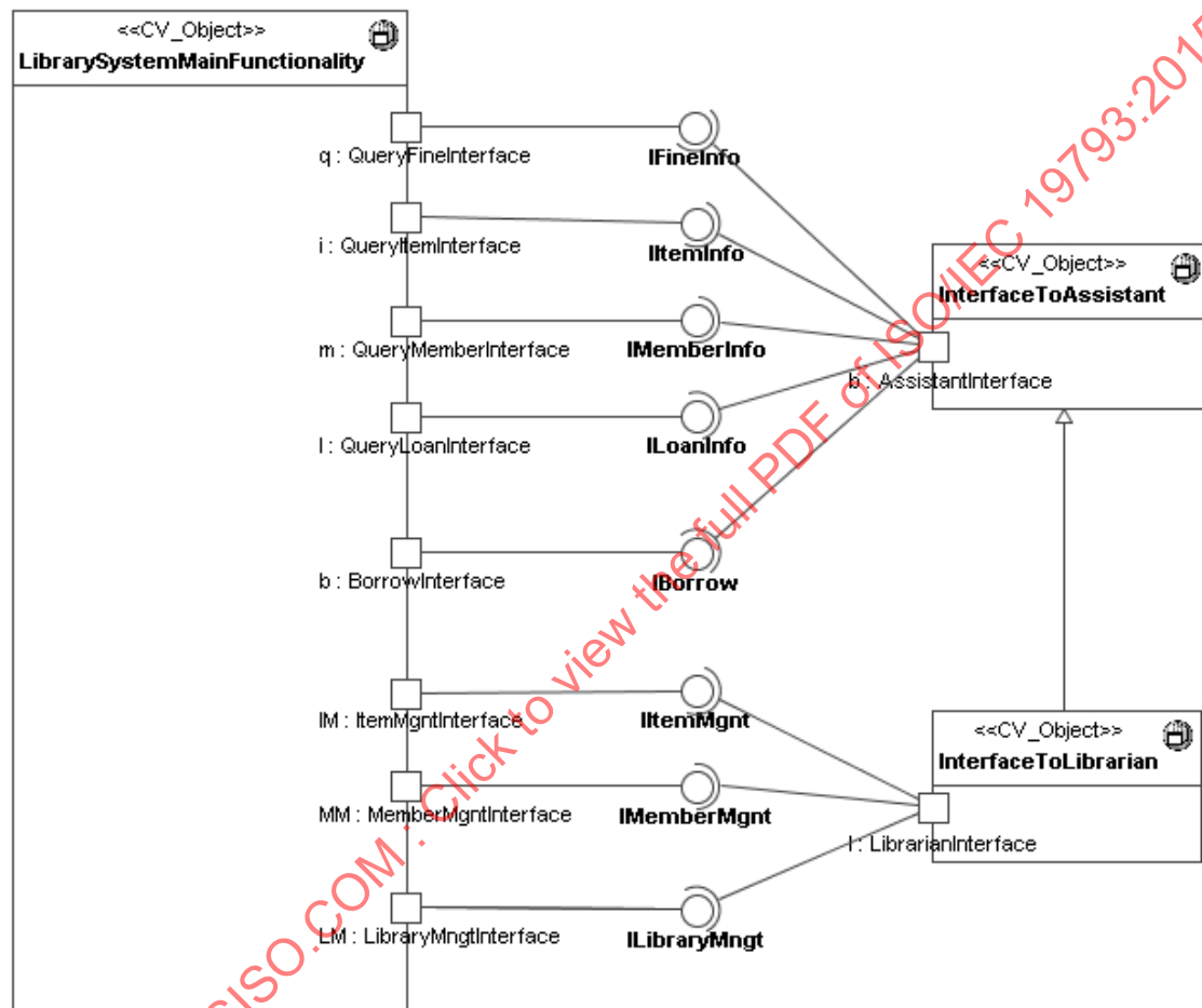
Figure A.29 – Component diagram with computational object templates and interface signatures of the system
