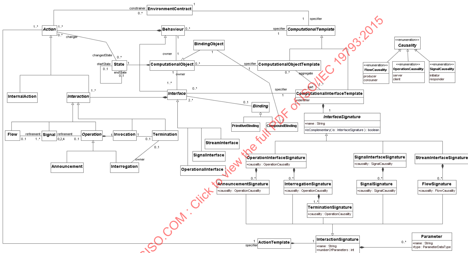
Figure 19 – Computational language concepts
