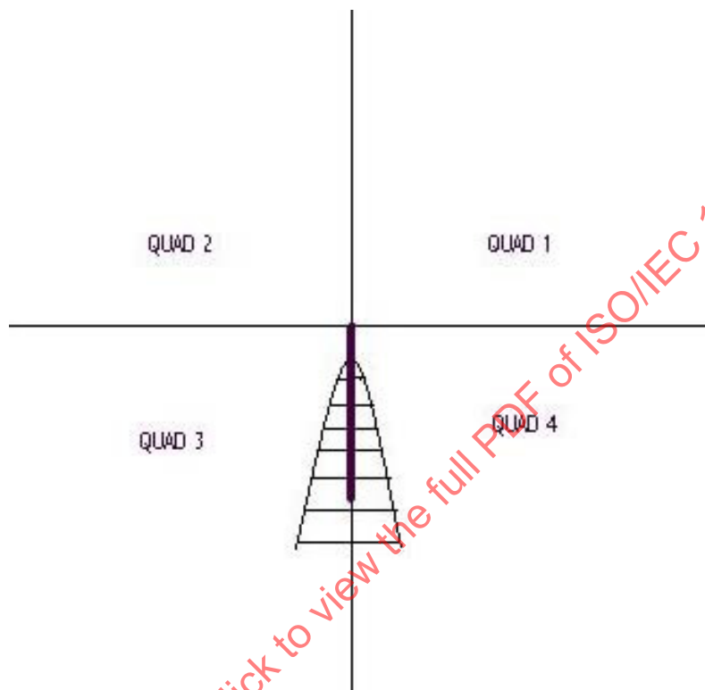
Figure 9 — Four-minutiae neighbourhood
