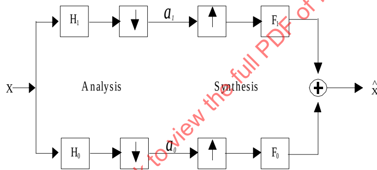
Figure E.2 — Two-Channel subband coder
