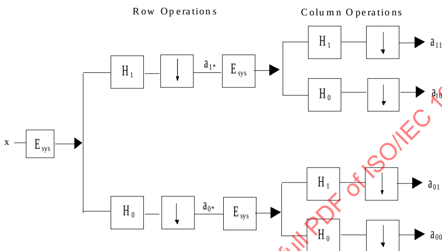
Figure E.4 — Single-Level, two-dimensional subband analysis
