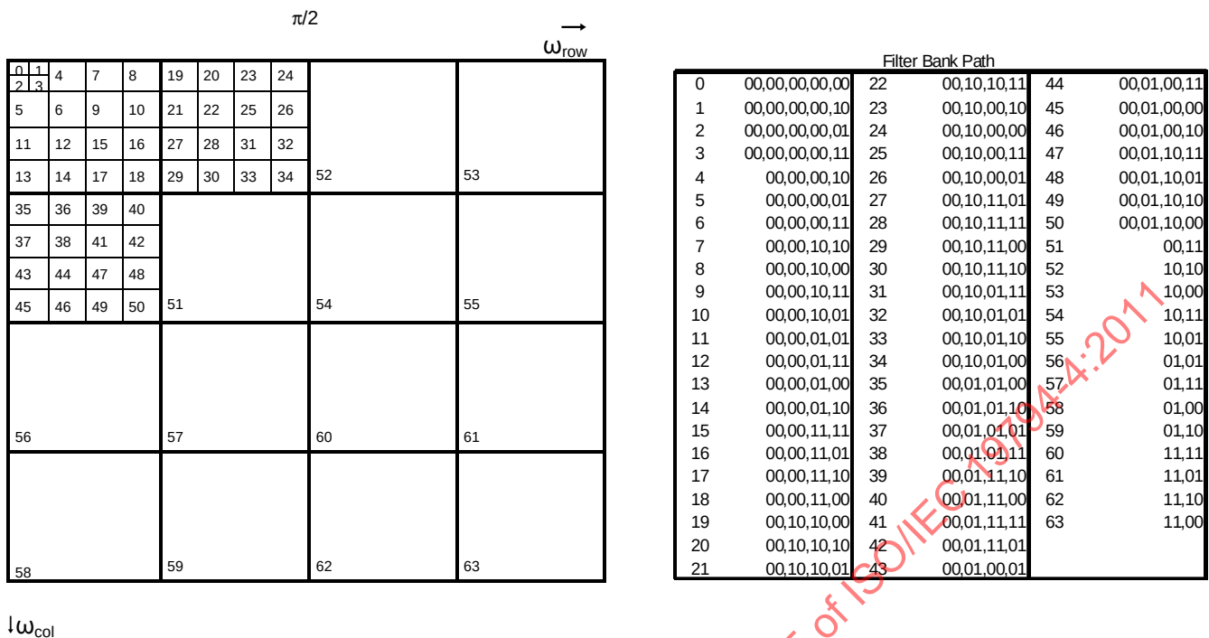
Figure E.6 — Subband decomposition
