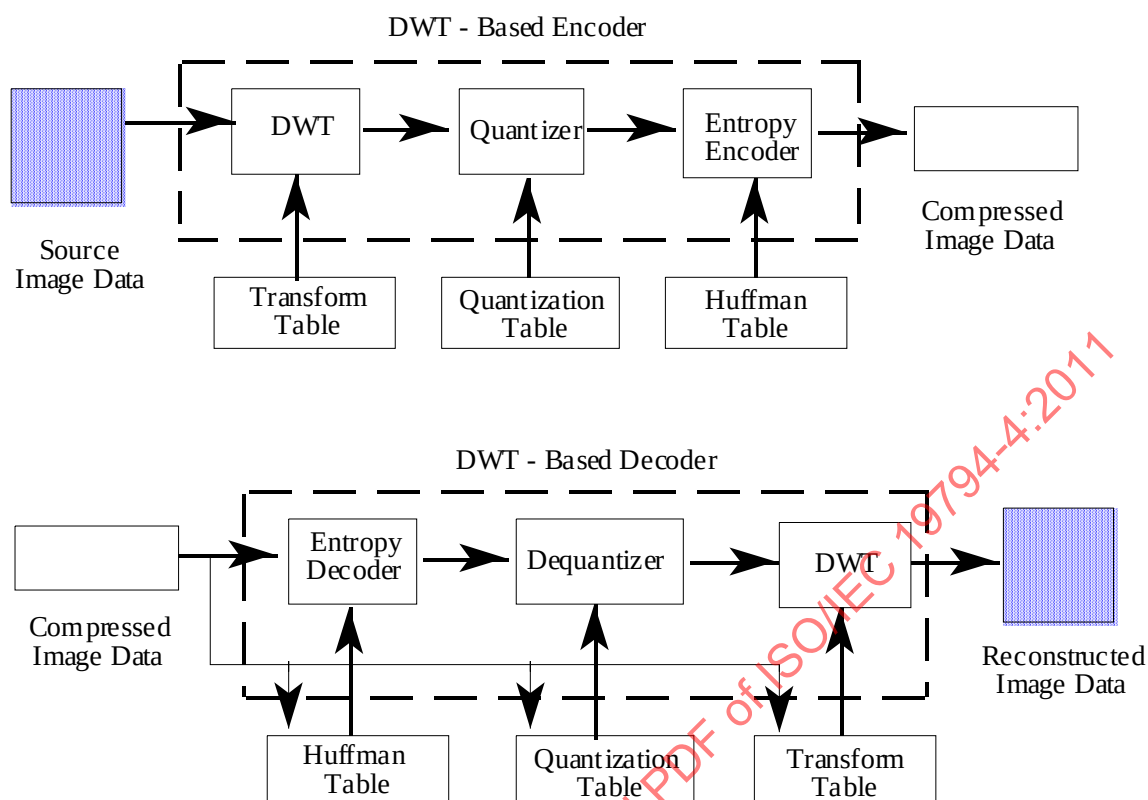
Figure E.1 — DWT-based encoder and decoder simplified diagram
