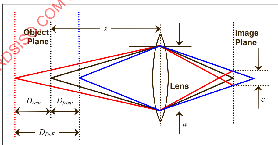
Figure C.1 — Dimensions for depth-of-field calculations
