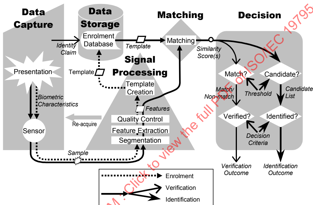
Figure 1 — Components of general biometric system
