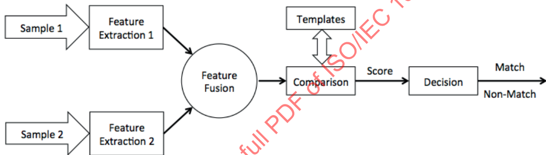
Figure F.5 — Fusion on the feature level
