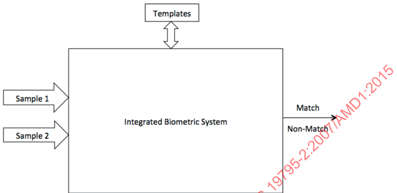
Figure F.2 — Fusion in an integrated multimodal system with decision output
