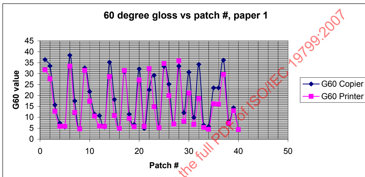
Figure B.1 — Substrate gloss ~ 4.4.
