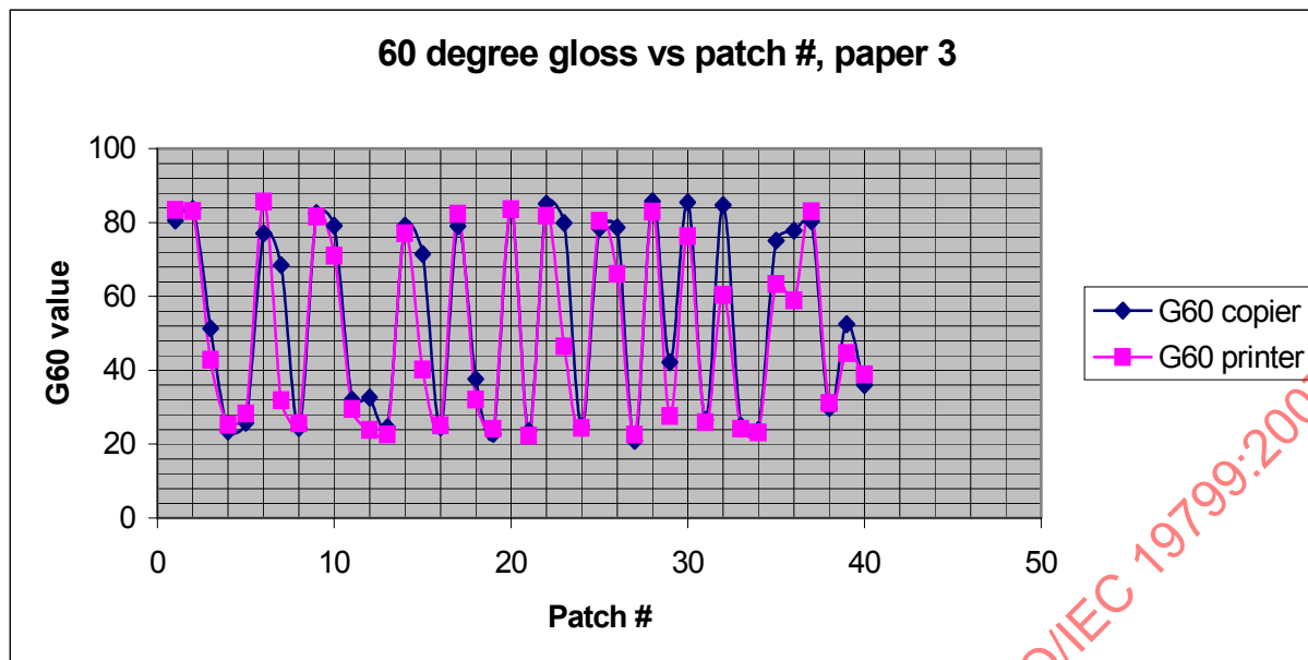
Figure B.3 — Substrate G60 ~36
