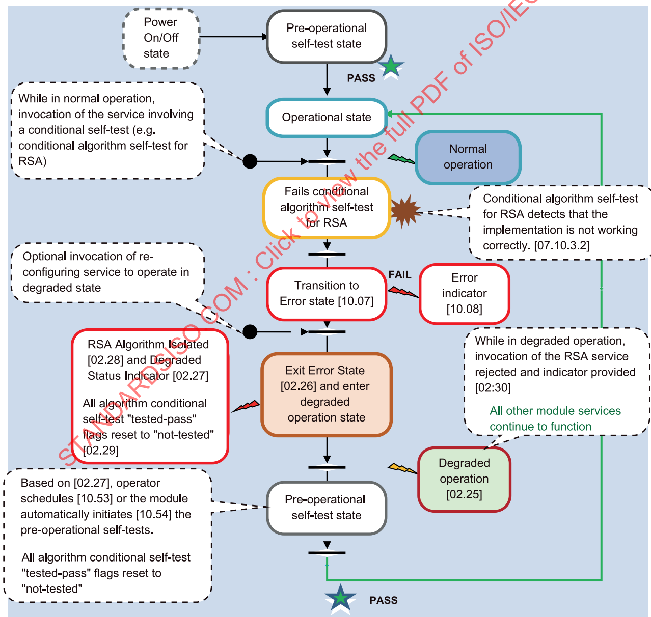
Figure C.2 — Example of state transitions supporting degraded functionality
