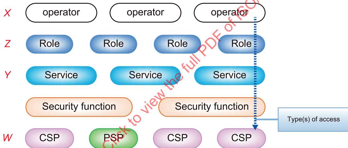
Figure C.5 — Overview of access control policy
