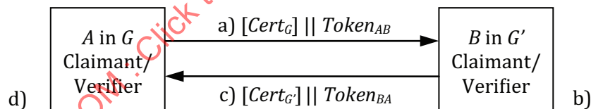
Figure 4 — Two-pass mutual anonymous authentication
