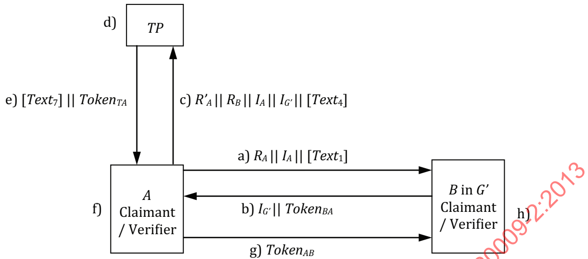
Figure 19 — Five-pass unilateral-anonymous mutual authentication initiated by A and B is anonymous
