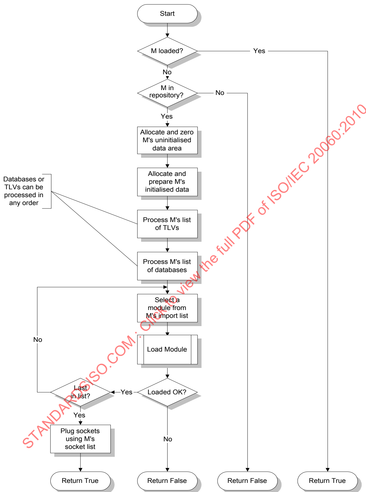
Figure 7-3 — Module loading procedure
