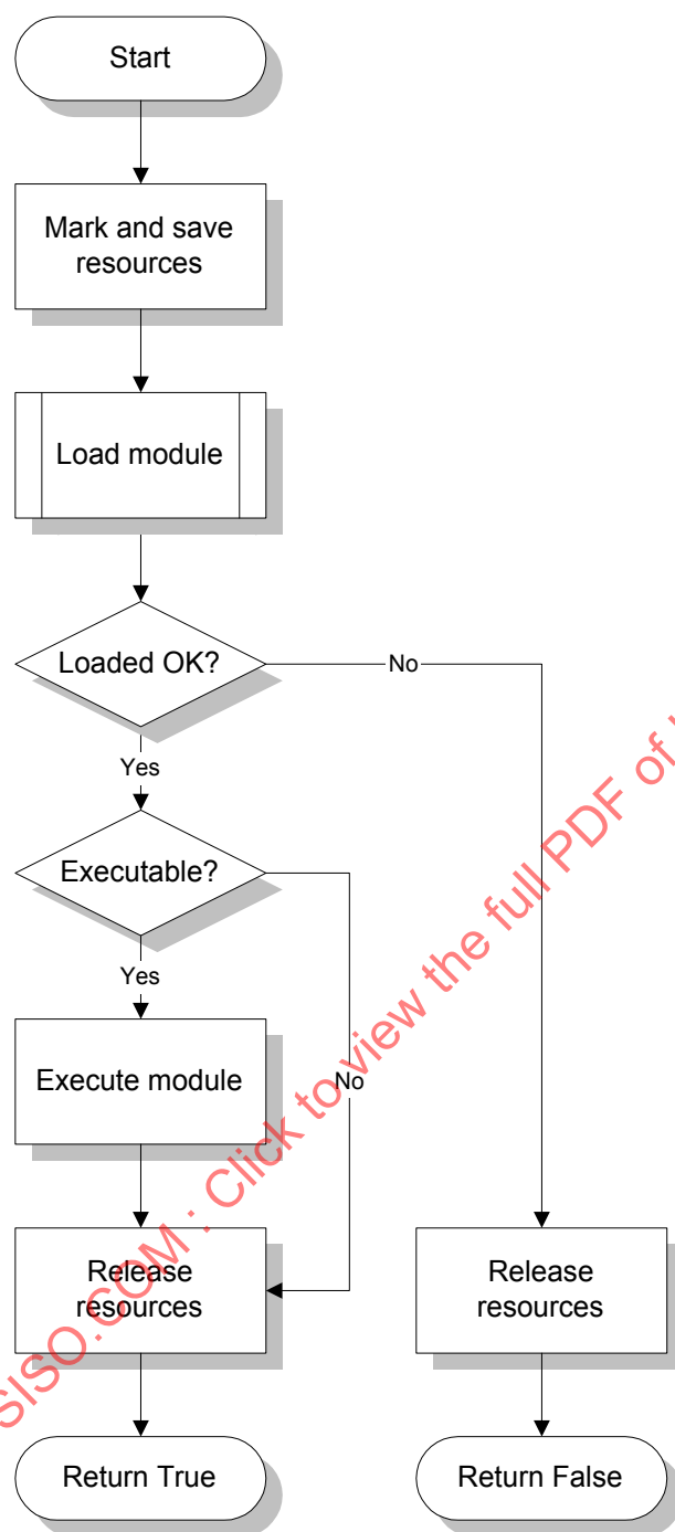
Figure 7-2 — Module execution procedure
