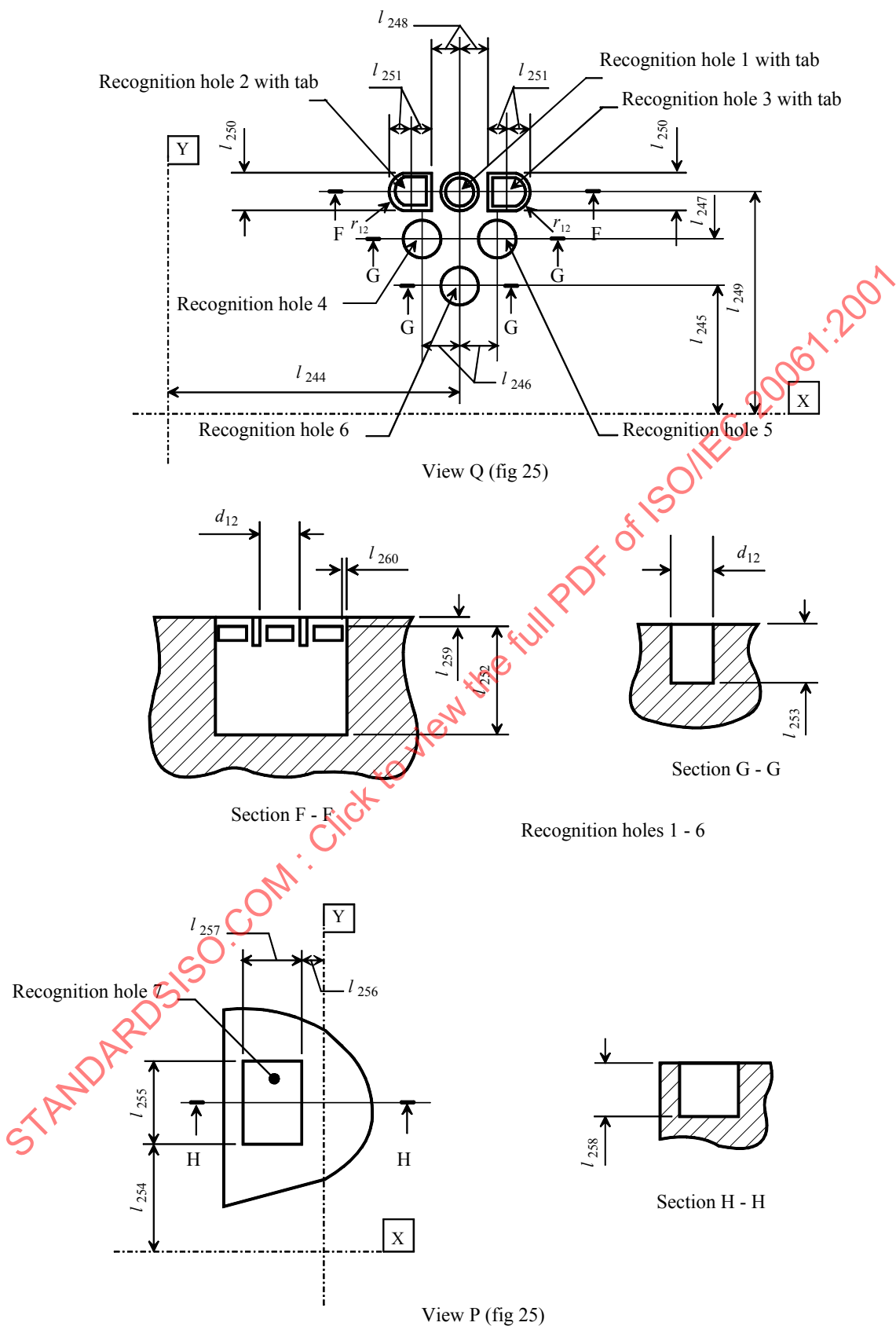
Figure 26 — Details of recognition holes of Type L cassette
