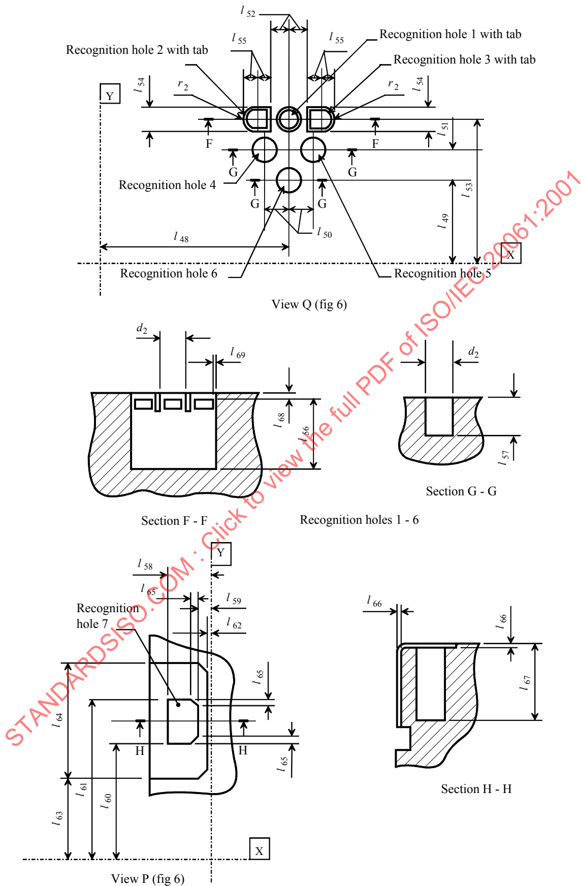
Figure 7 — Details of recognition holes of Type S cassette
