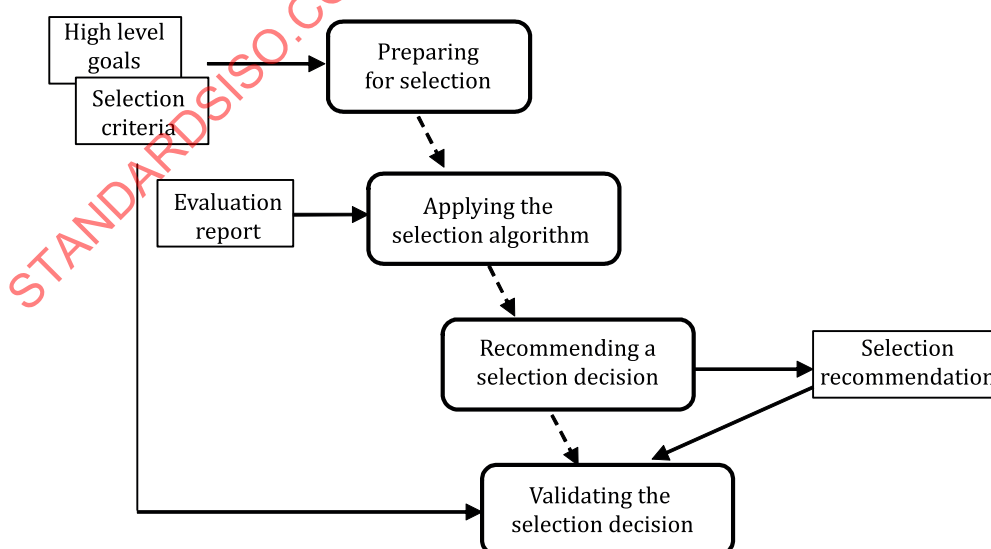
Figure 5 — Overview of selection process
