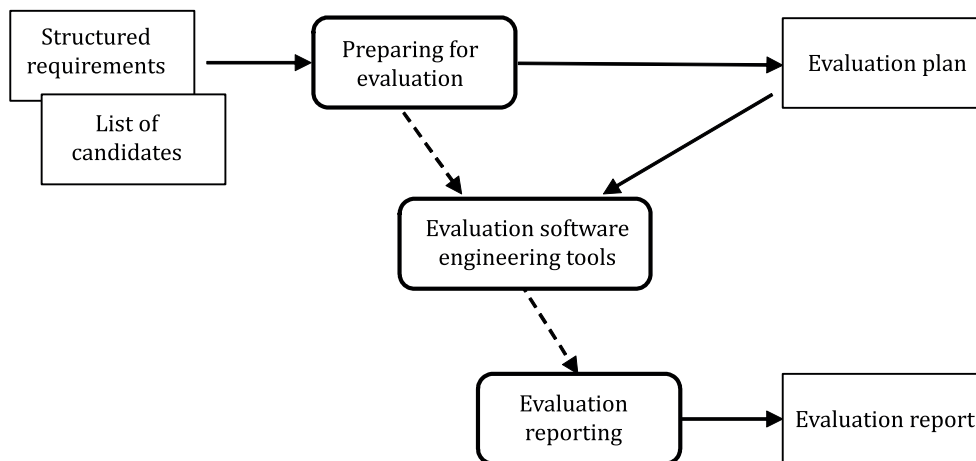
Figure 4 — Overview of evaluation process
