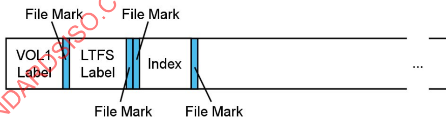
Figure 4 — Partition Layout
