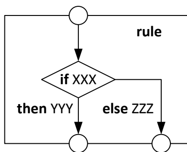
Figure 4 — branch rule
