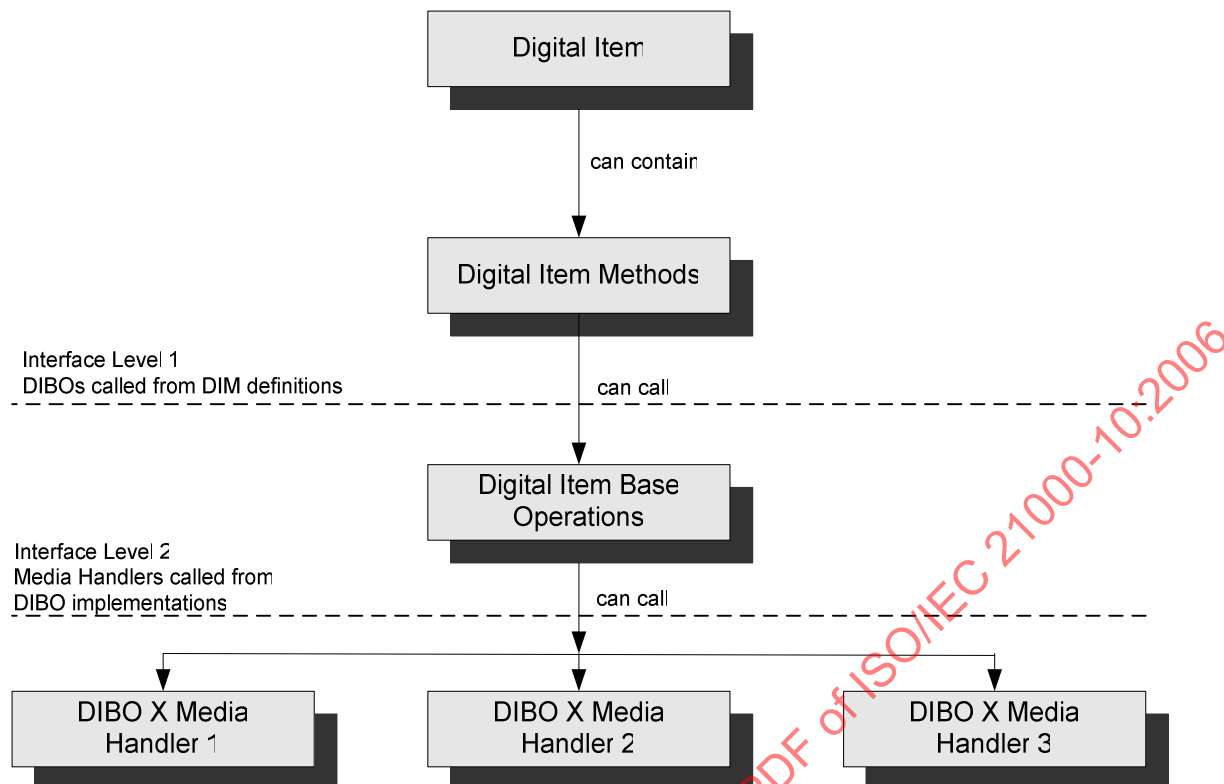
Figure F.1 — DIBO implementation using media handlers
