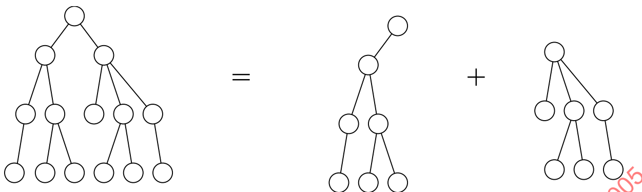
Figure 1 — Decomposition of a description into two description fragments
