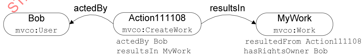
Figure A.1 — Three individuals in the Ontology
