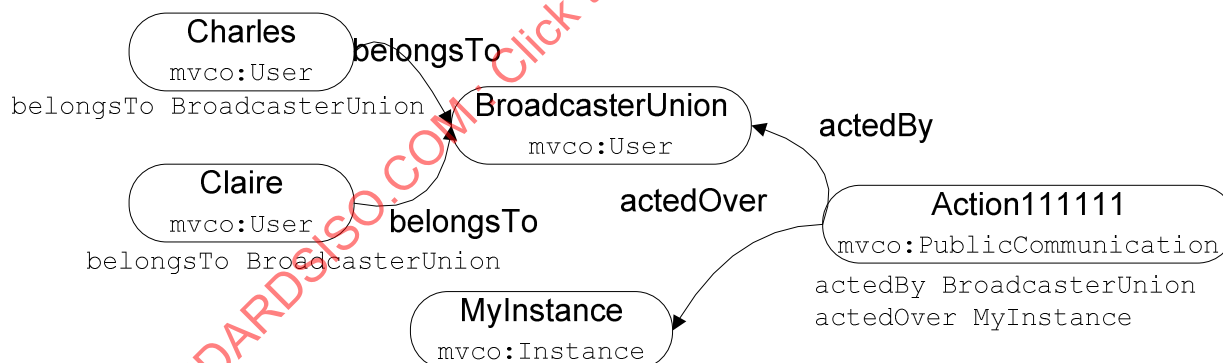
Figure A.3 — Alice's Instance is broadcasted
