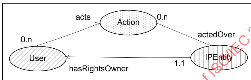
Figure 1 — Relations between Actions, Users and IP Entities
