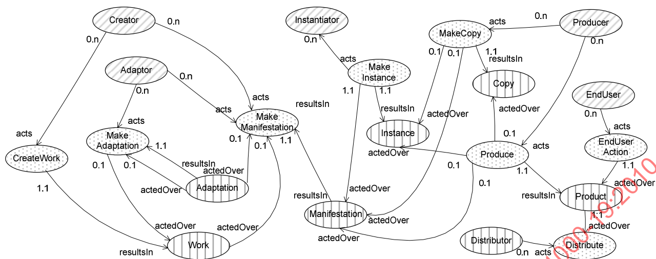
Figure 3 — Diagram of classes connected by the relationships “acts”, “actedOver” and “resultsIn”
