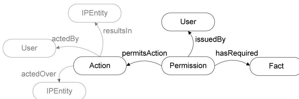
Figure 5 — Relations of Permissions with other MVCO elements
