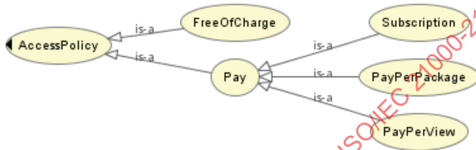
Figure 27 — Subclasses of mco-ipre:AccessPolicy
