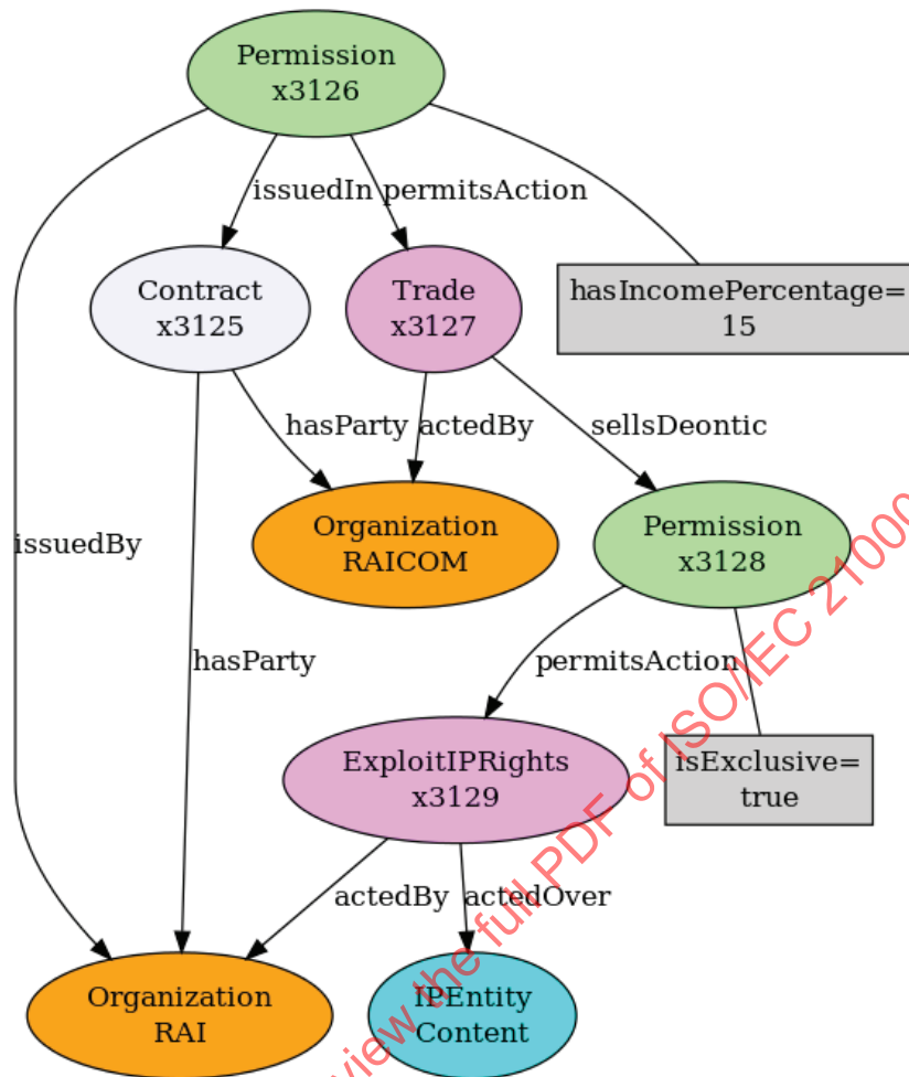
Figure 17 — Example of permission for trade of rights (mandate)
