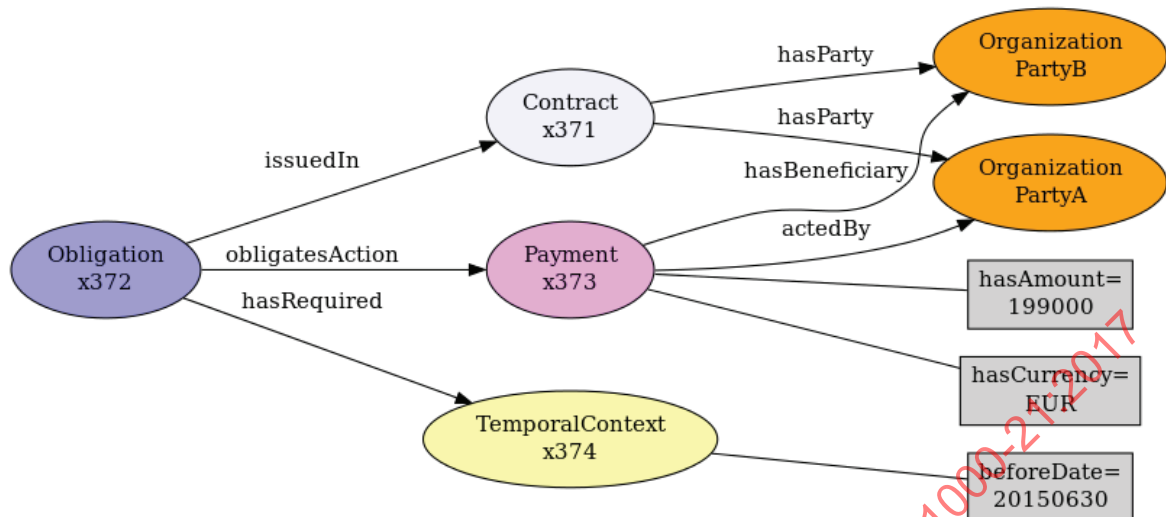
Figure 20 — Example of obligation of payment for a defined amount
