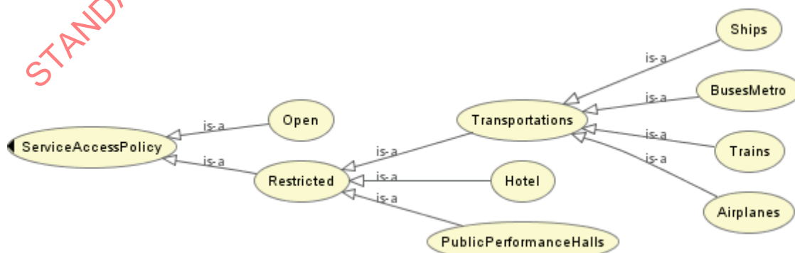
Figure 31 — Subclasses of mco-ipre:ServiceAccessPolicy
