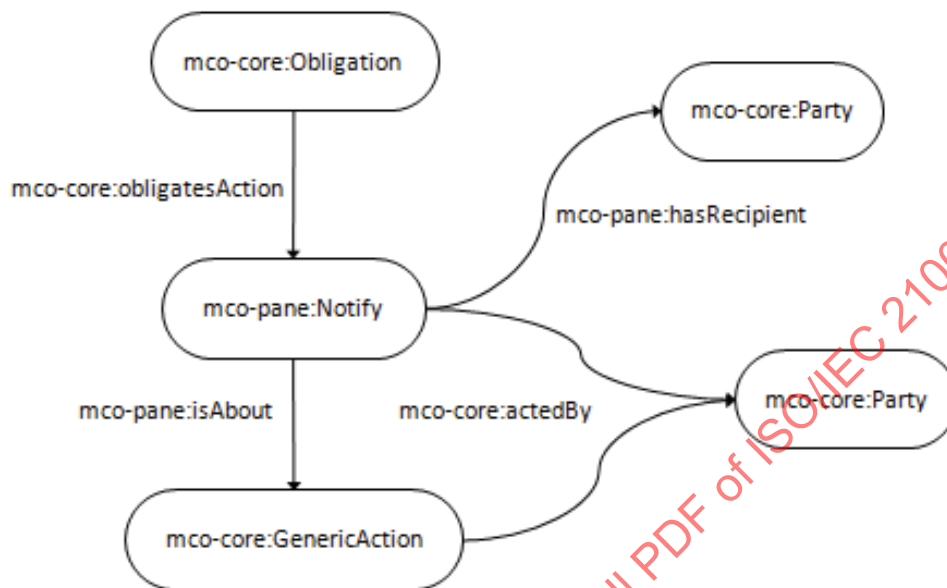
Figure 19 — Classes and object properties around notify action
