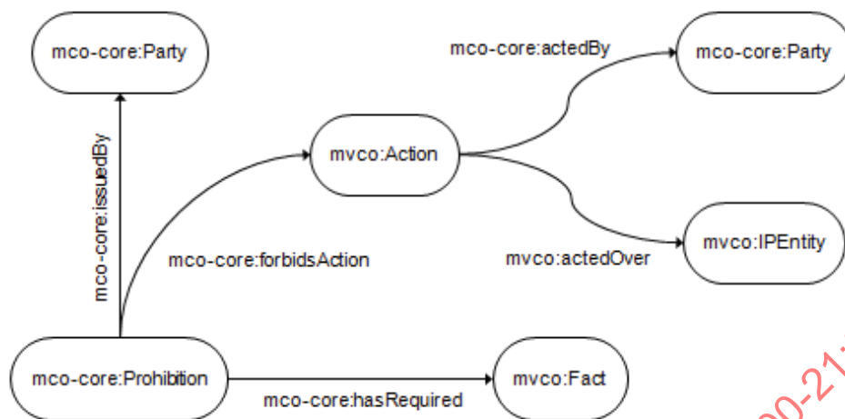
Figure 9 — Classes and object properties around prohibition
