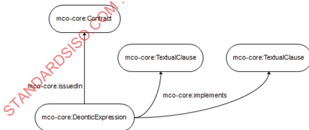
Figure 8 — Classes and object properties around textual clauses
