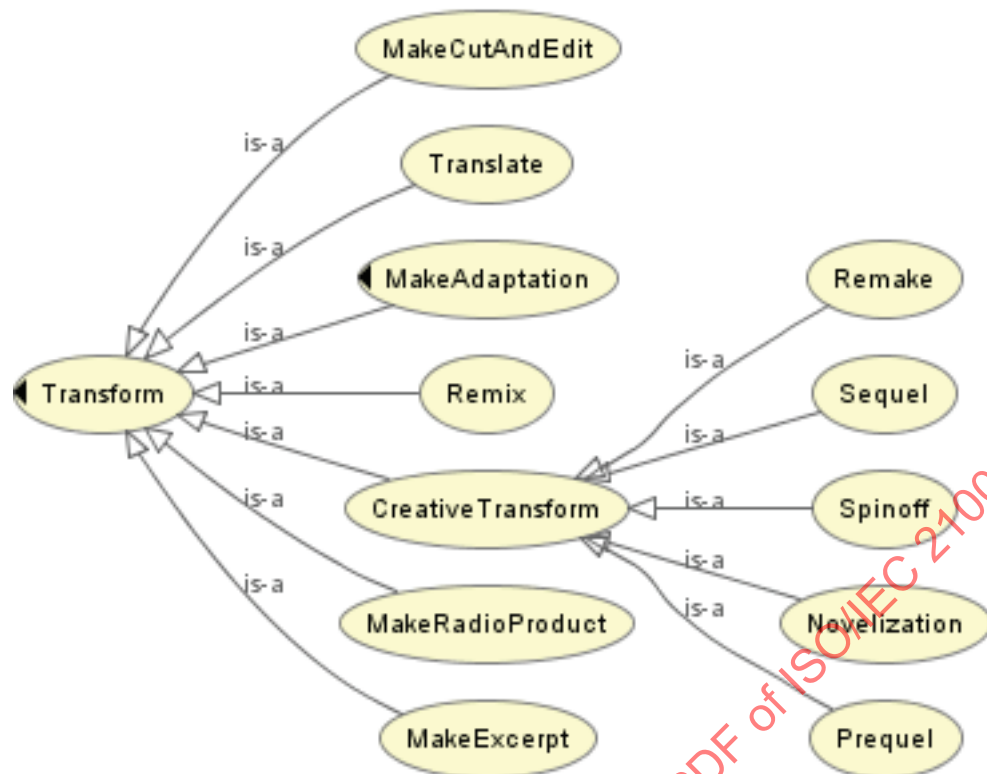
Figure 25 — Subclasses of mco-ipre:Transform
