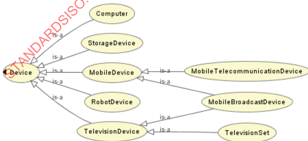
Figure 29 — Subclasses of mco-ipre:Device
