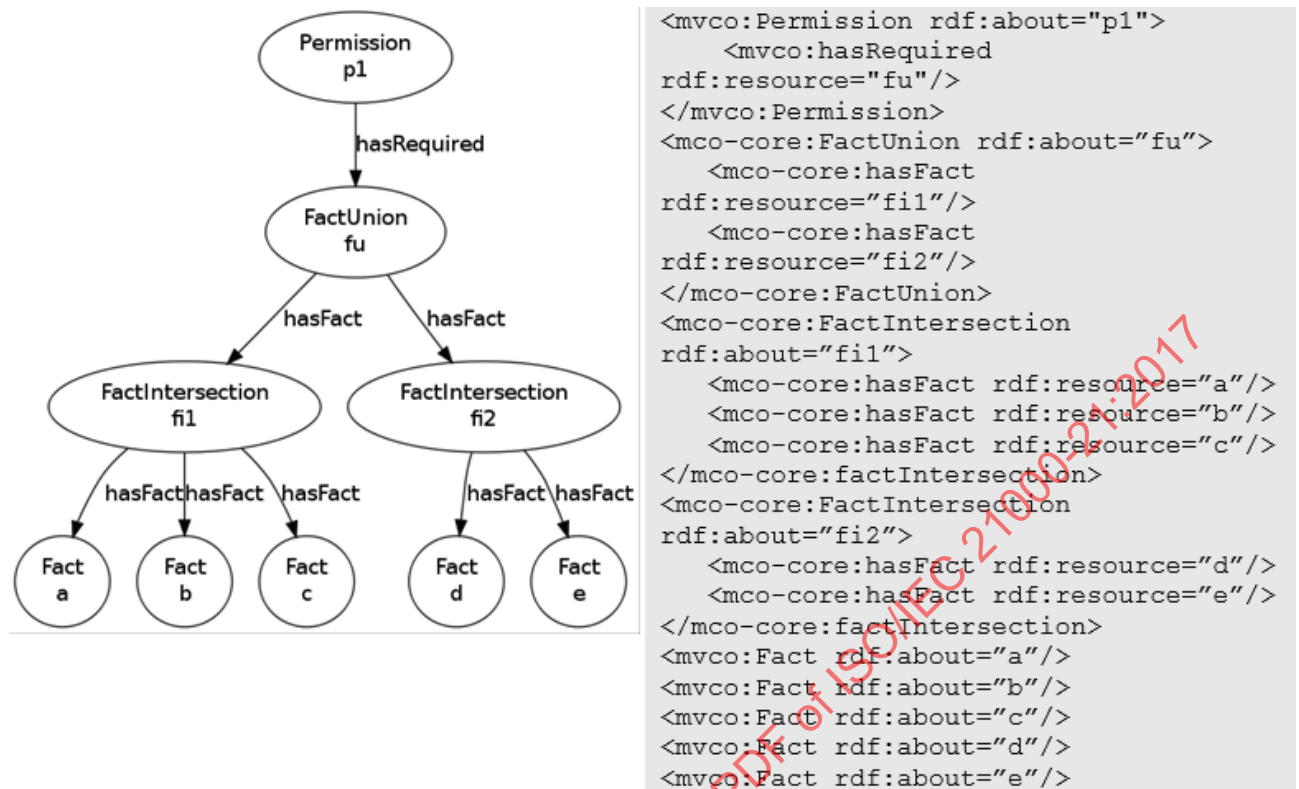
Figure 14 — Diagram and RDF/XML excerpt of a fact composition example
