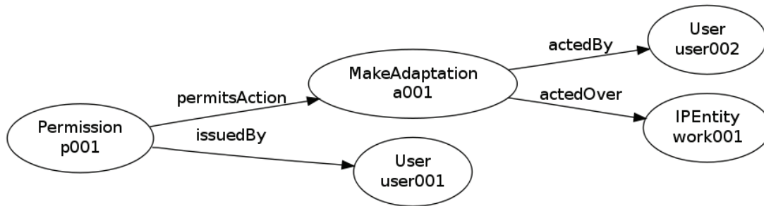
Figure 11 — Simple example of permission
