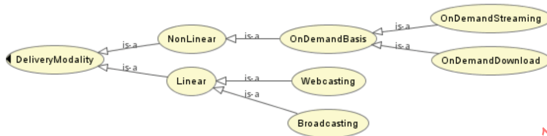
Figure 28 — Subclasses of mco-ipre:DeliveryModality
