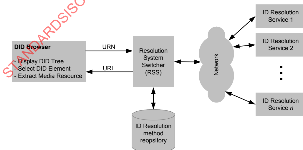
Figure B.2 — An Implementation Example: Resolution System Switcher (RSS)
