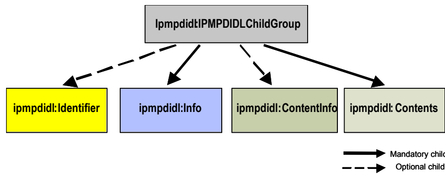
Figure 2 — Structure of IPMP DIDL elements for the DID model
