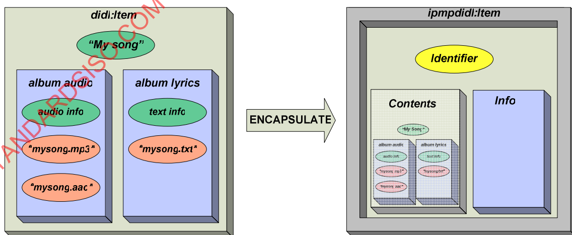
Figure D.2 — IPMP DIDL processing example
