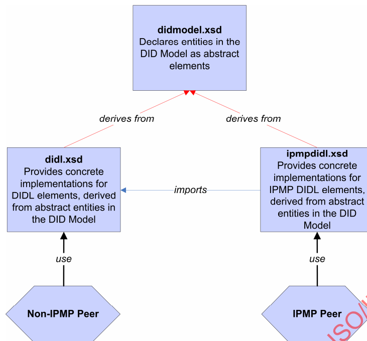
Figure 1 — Schema relationship between DID model, DIDL and IPMP DIDL
