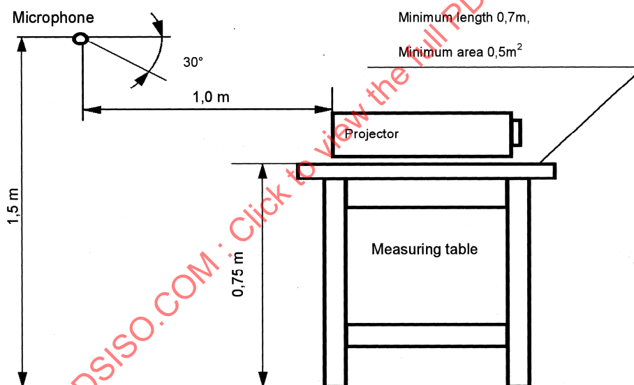
Figure B.3 — Acoustic Noise measuring procedure
