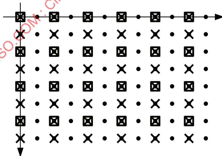
Figure B.1 — Sampling grid for 4:2:2 sampling
