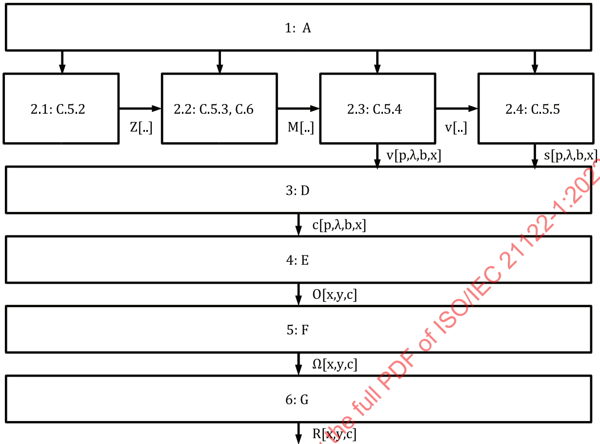
Figure 2 — Decoder overview
