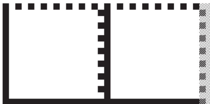
Figure F.5 — External clock track segment
