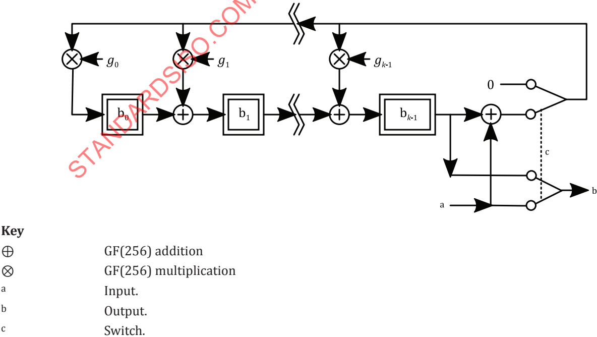
Figure 5 — Error correction codeword encoding circuit
