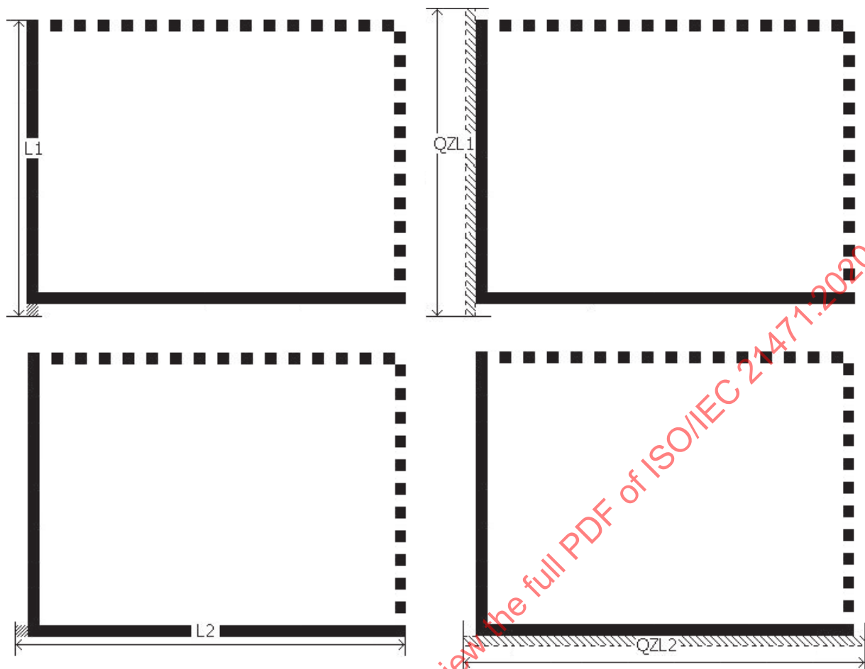
Figure F.1 — Outside L and corresponding quiet zone segments of fixed pattern
