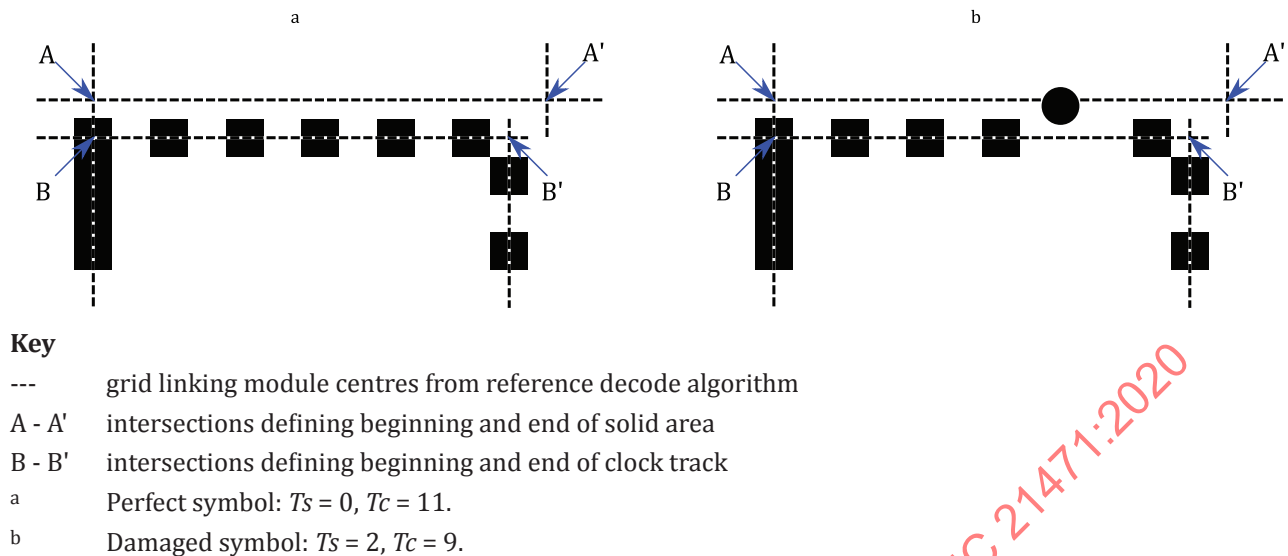
Figure F.3 — Transitions in perfect symbol (left) and damaged symbol (right)
