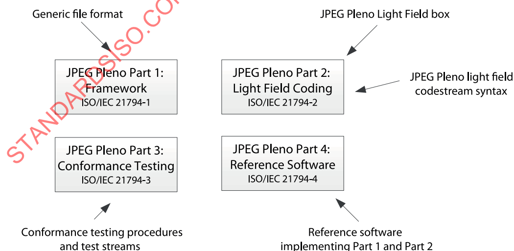
Figure 1 — JPEG Pleno framework
