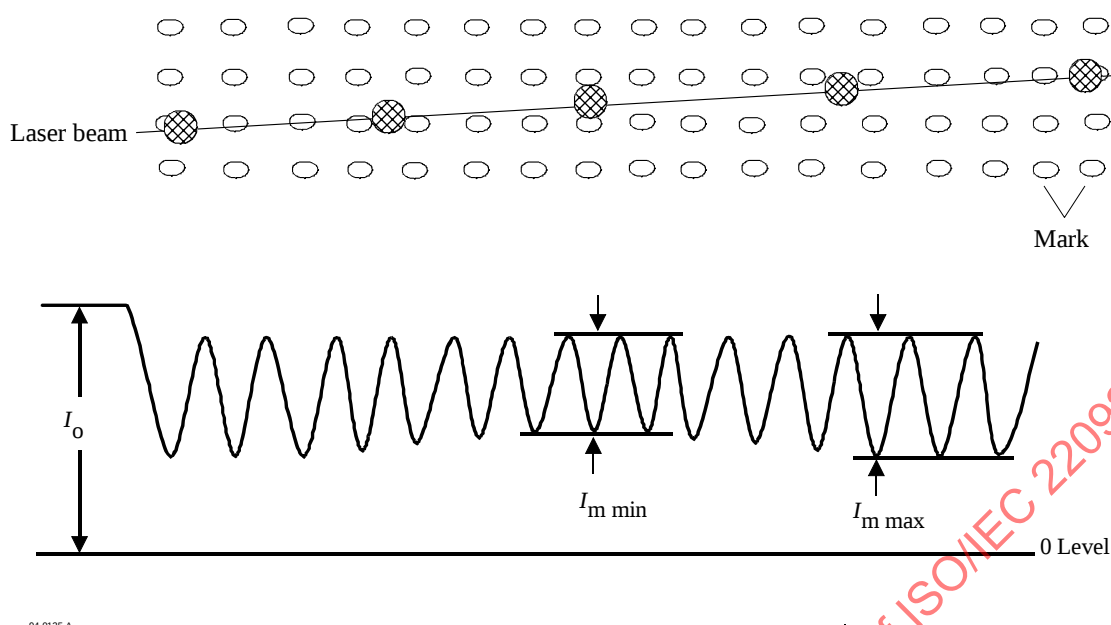
Figure 25 - Path of the laser beam when crossing tracks and the resulting PEP signals
