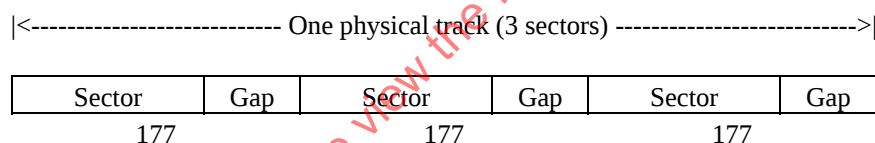
Figure 22 - Track format in the PEP Zone
