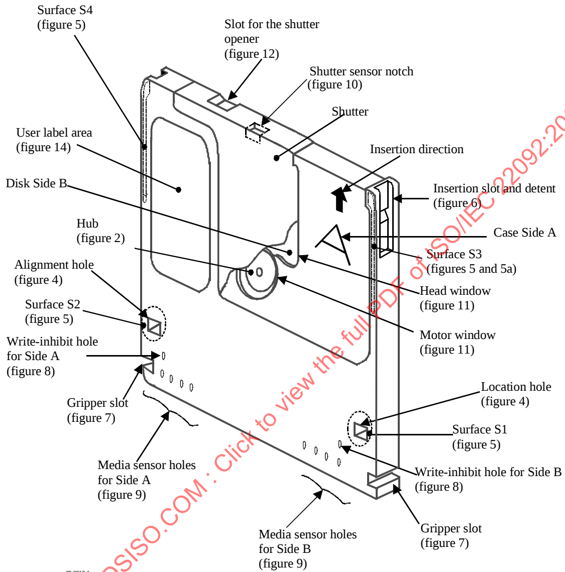
Figure 3 - Case
