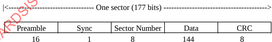
Figure 23 - Sector format in the PEP Zone
