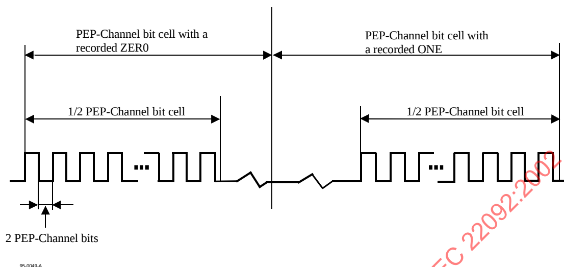
Figure 21 - Example of phase-encoded modulation in the PEP Zone
