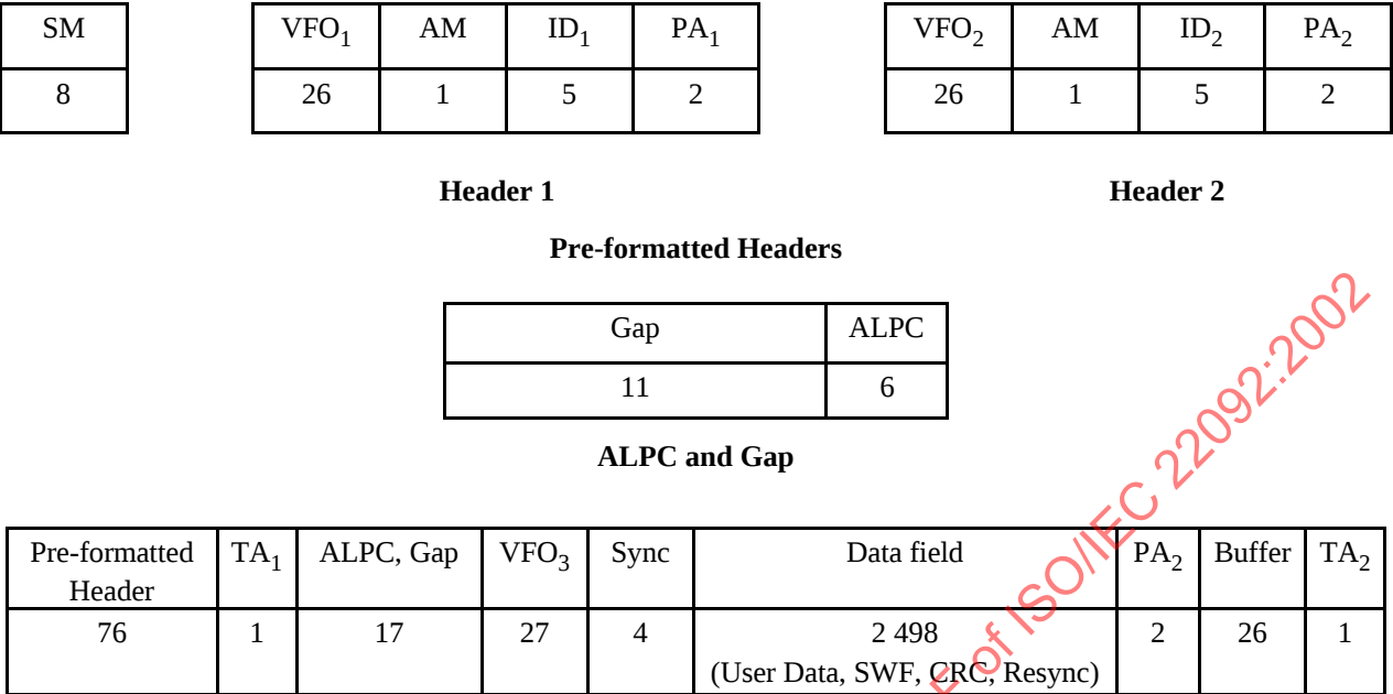
Figure 17 - Sector format for 2 048 user bytes
