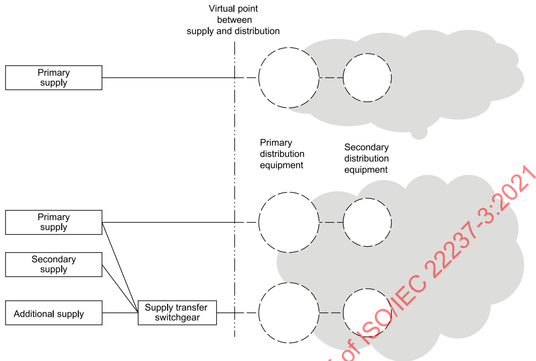
Figure 2 — Power supply functional elements
