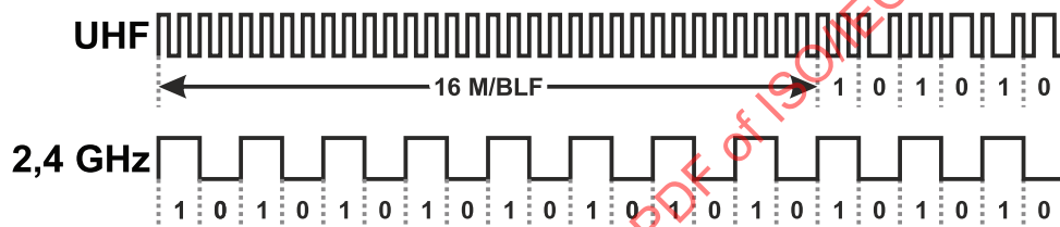
Figure 6 — UHF and 2,4 GHz backscatter alignment (Example A and Example B)
