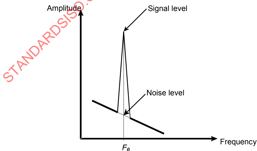
Figure 25 – Spectrum analyzer display
